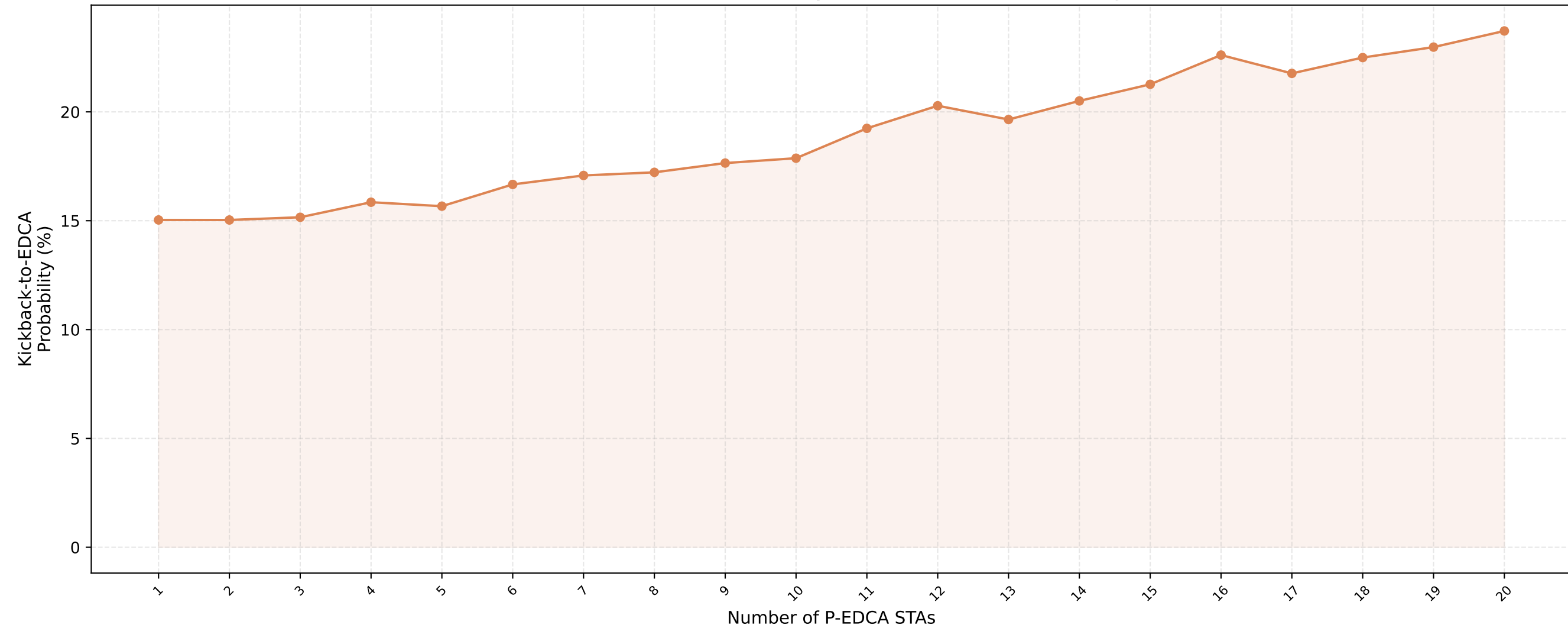
[Stat 5] P-EDCA Kickback Probability — nSta=20, 1Mbps (avg of 10 runs)
