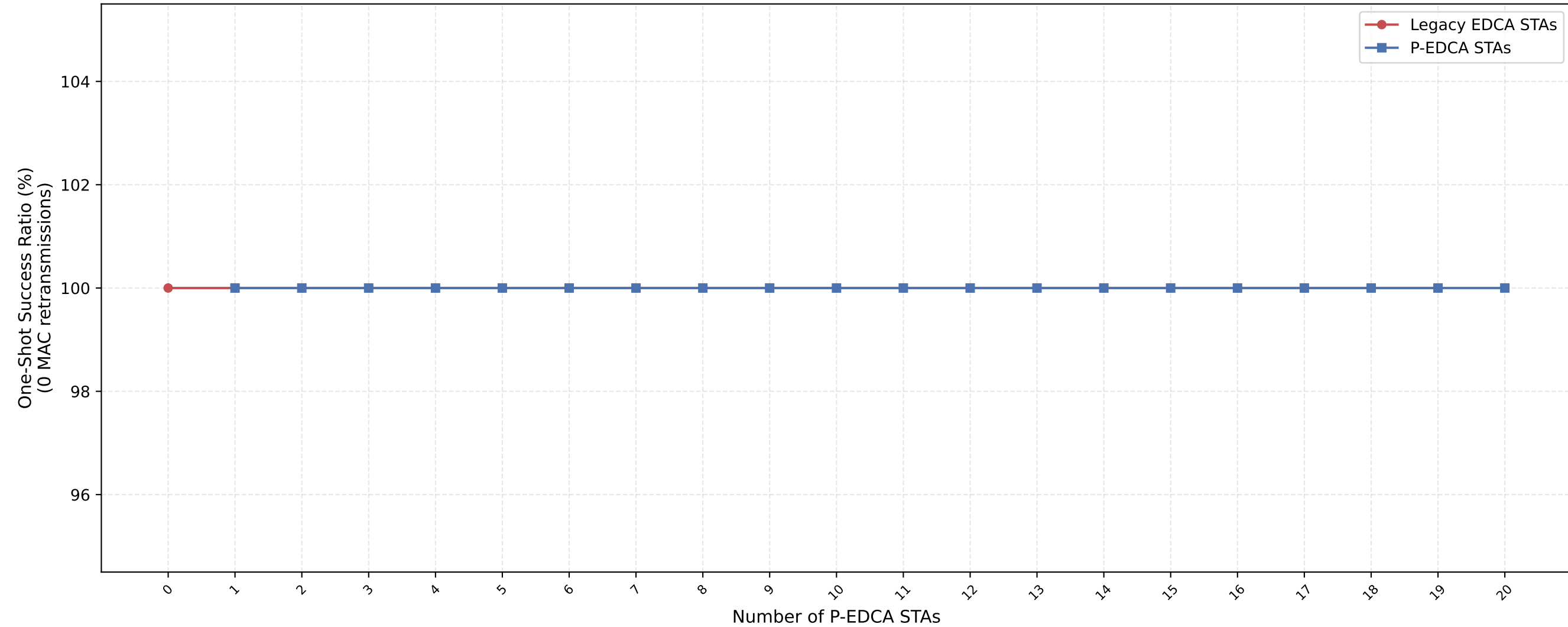
EDCA One-Shot Success Ratio (0 retx) — nSta=20, 1Mbps (avg of 10 runs)
