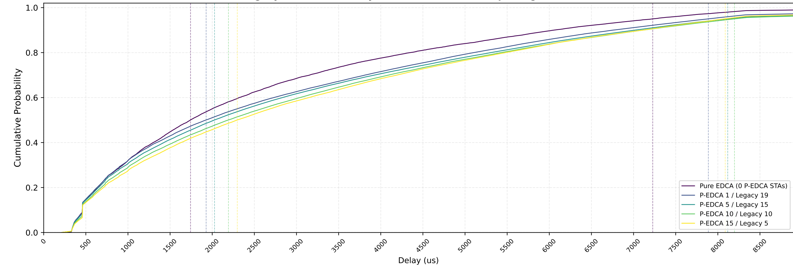
Legacy EDCA STAs Delay CDF — nSta=20, 1Mbps, avg of 10 runs
