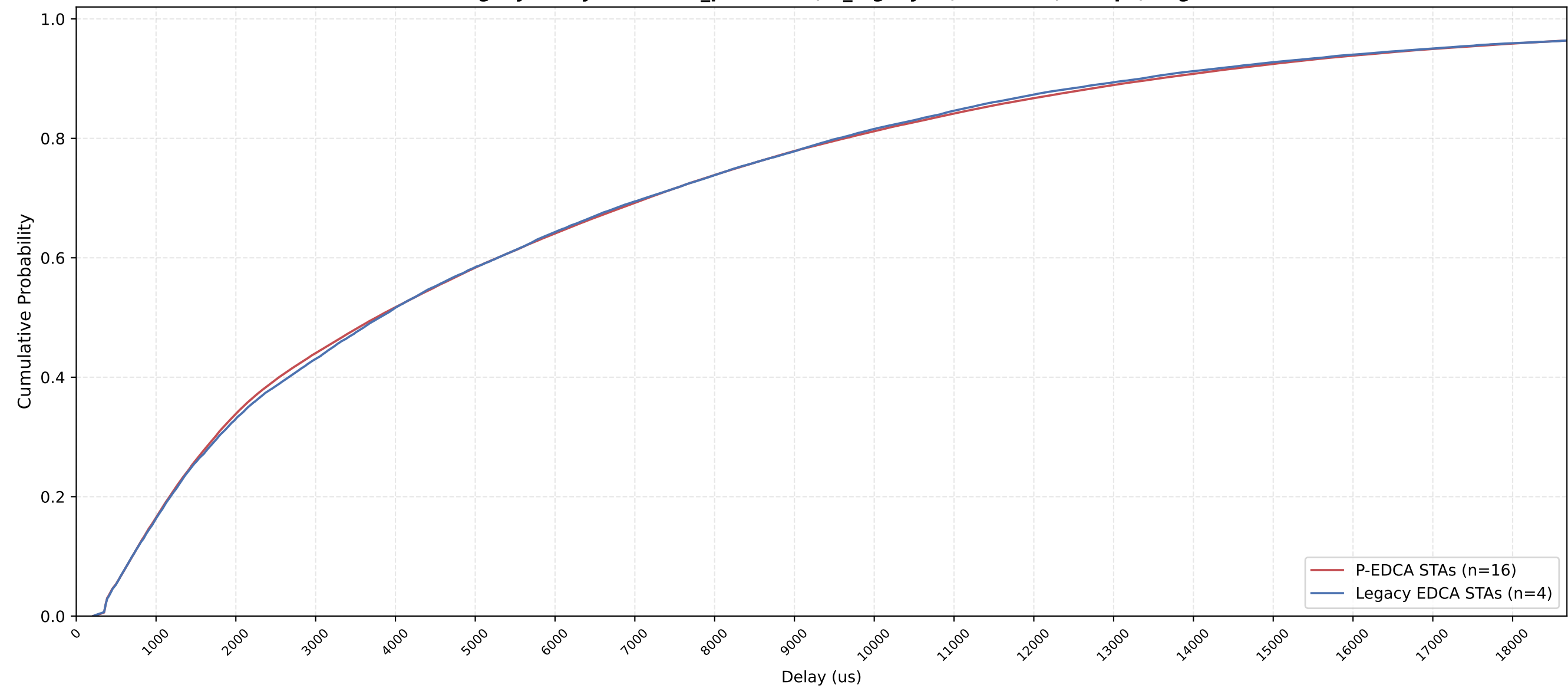
P-EDCA vs Legacy Delay CDF — n_pedca=16, n_legacy=4, nSta=20, 1Mbps, avg of 10 runs
