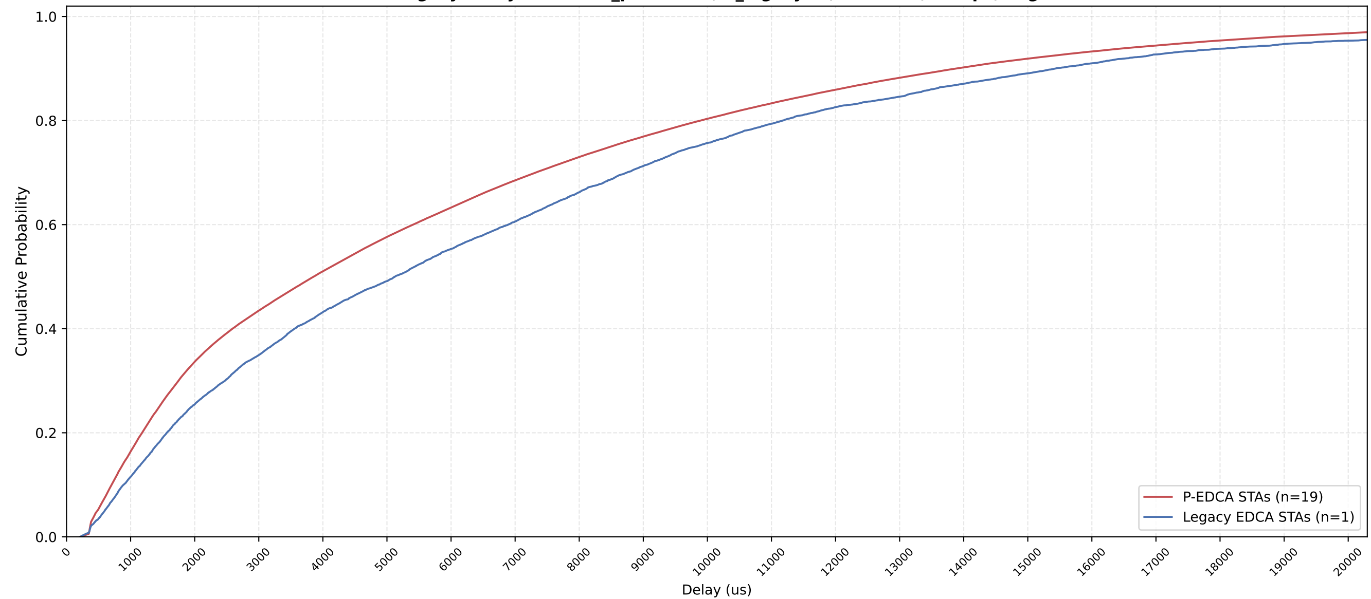
P-EDCA vs Legacy Delay CDF — n_pedca=19, n_legacy=1, nSta=20, 1Mbps, avg of 10 runs
