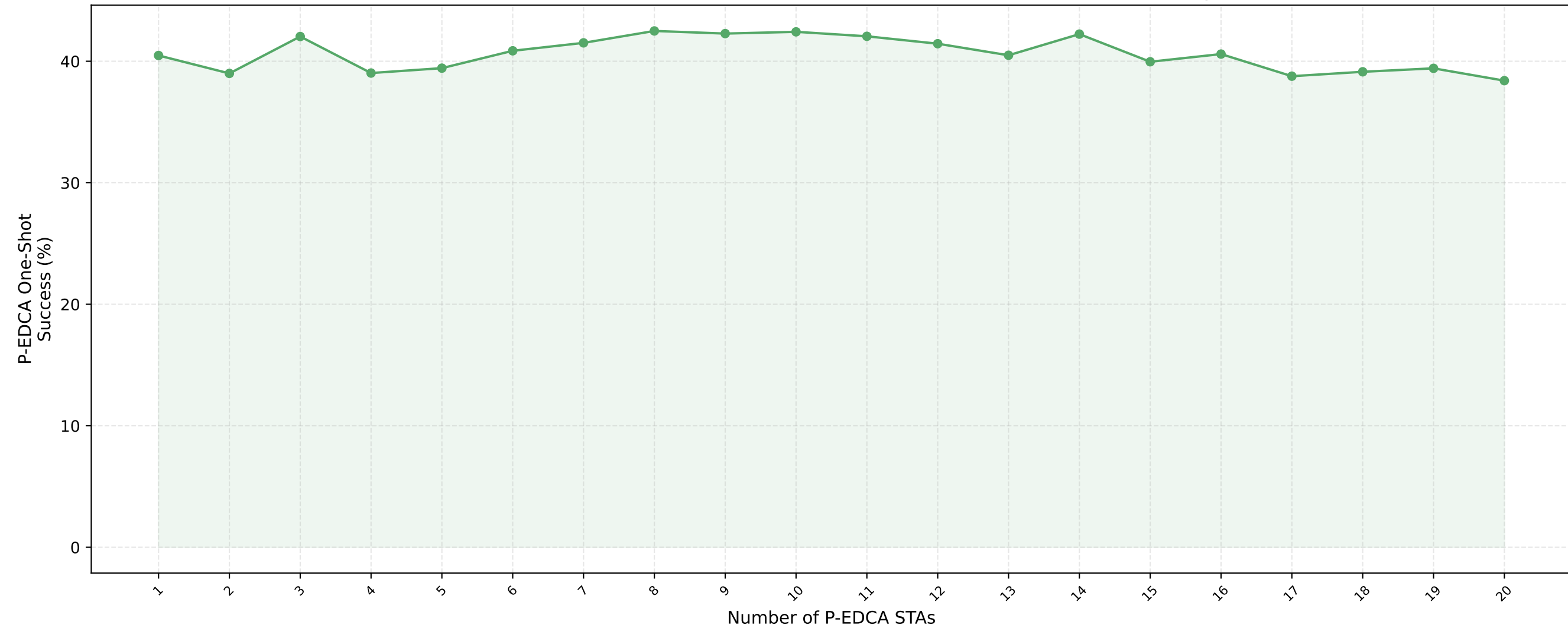
[Stat 3] P-EDCA One-Shot Success (Success/DS-CTS) — nSta=20, 1Mbps (avg of 10 runs)
