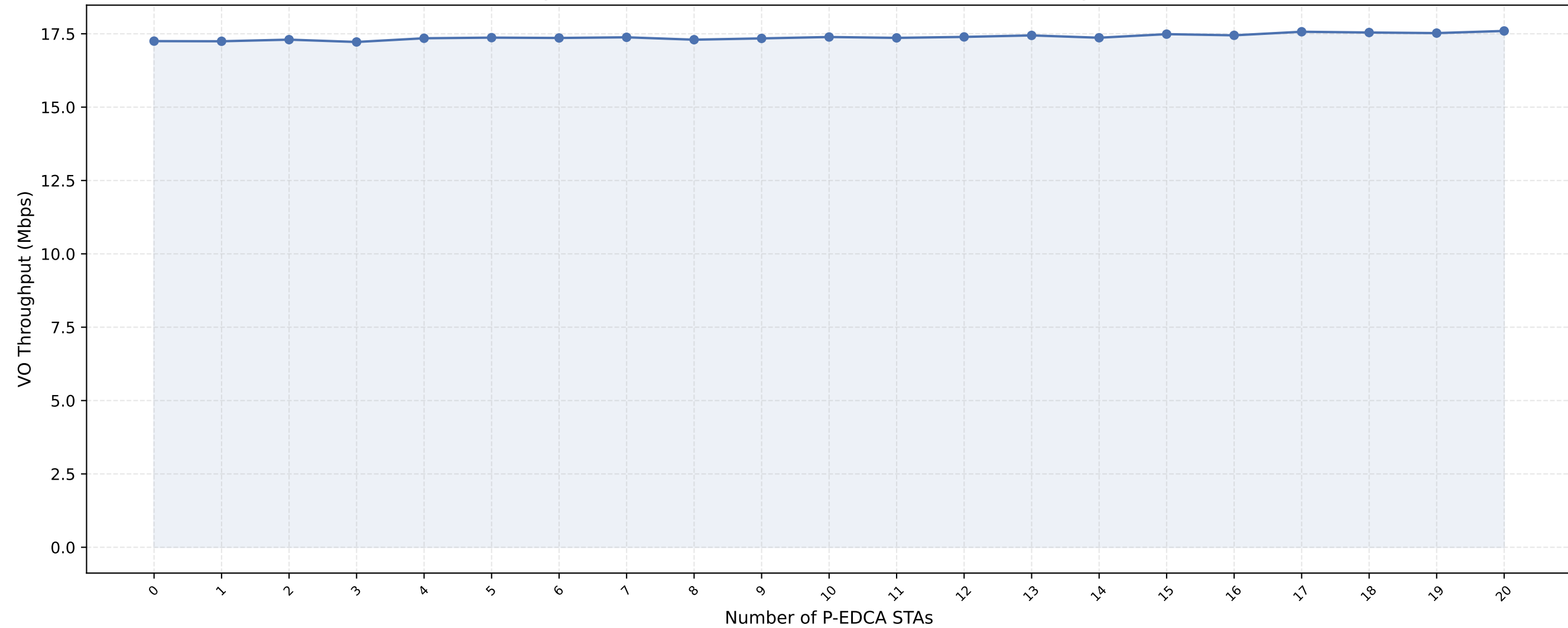
VO Throughput vs P-EDCA STAs — nSta=20, 1Mbps (avg of 10 runs)
