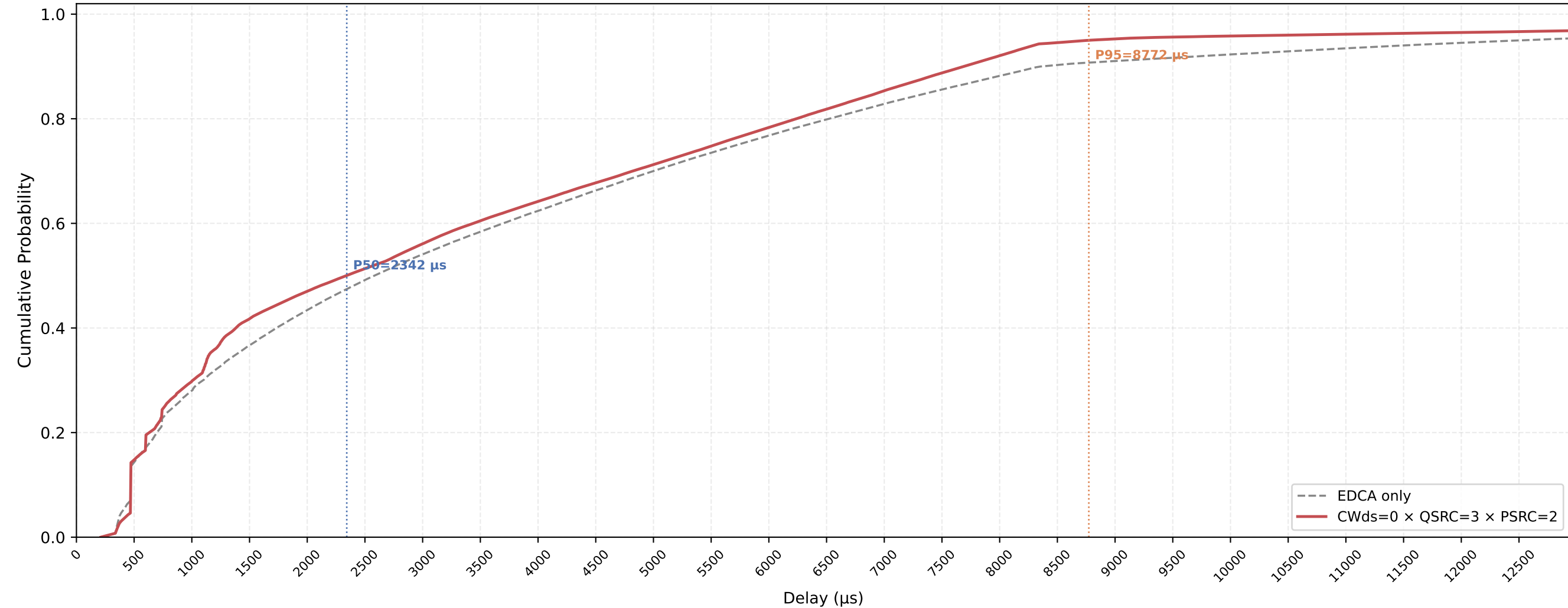
VO (all STAs) Delay CDF — CWds=0 × QSRC=3 × PSRC=2 nSta=30, nPedca=30, 1Mbps, avg of 10 runs
