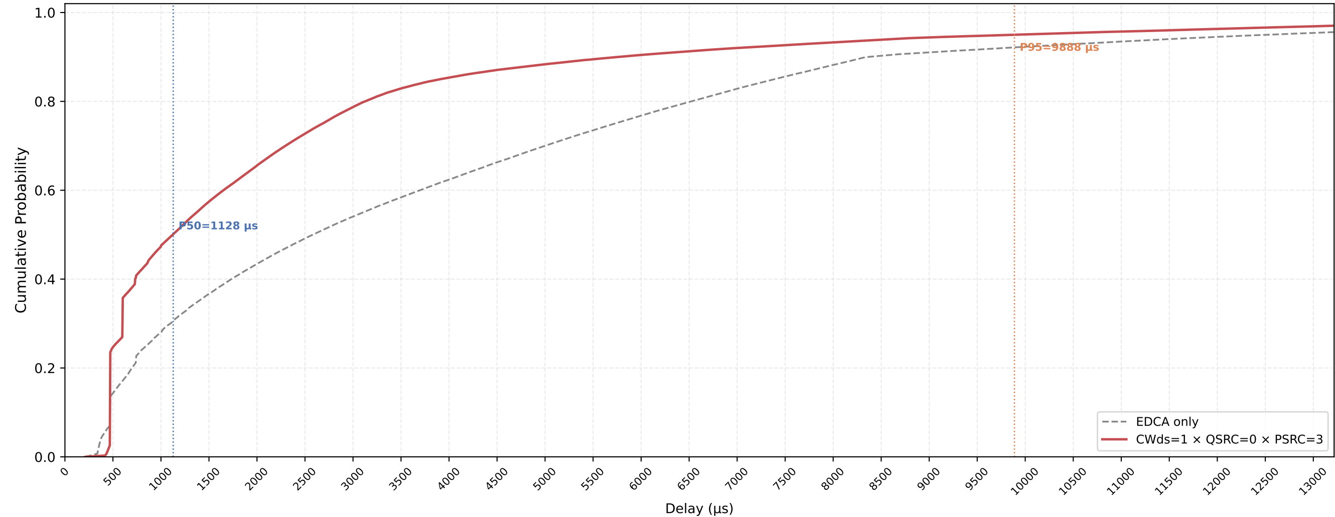
P-EDCA STA VO Delay CDF — CWds=1 × QSRC=0 × PSRC=3 nSta=30, nPedca=30, 1Mbps, avg of 10 runs
