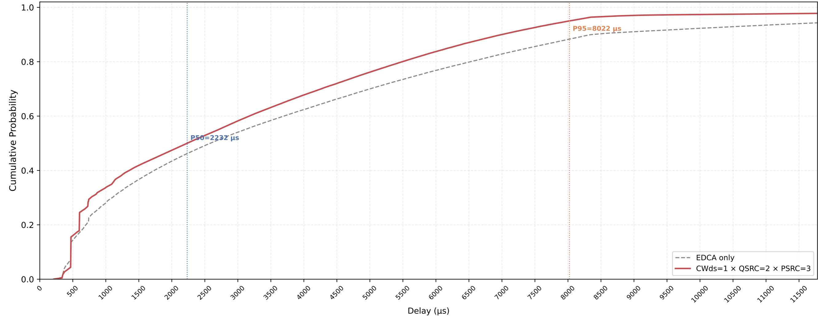
VO (all STAs) Delay CDF — CWds=1 × QSRC=2 × PSRC=3 nSta=30, nPedca=30, 1Mbps, avg of 10 runs
