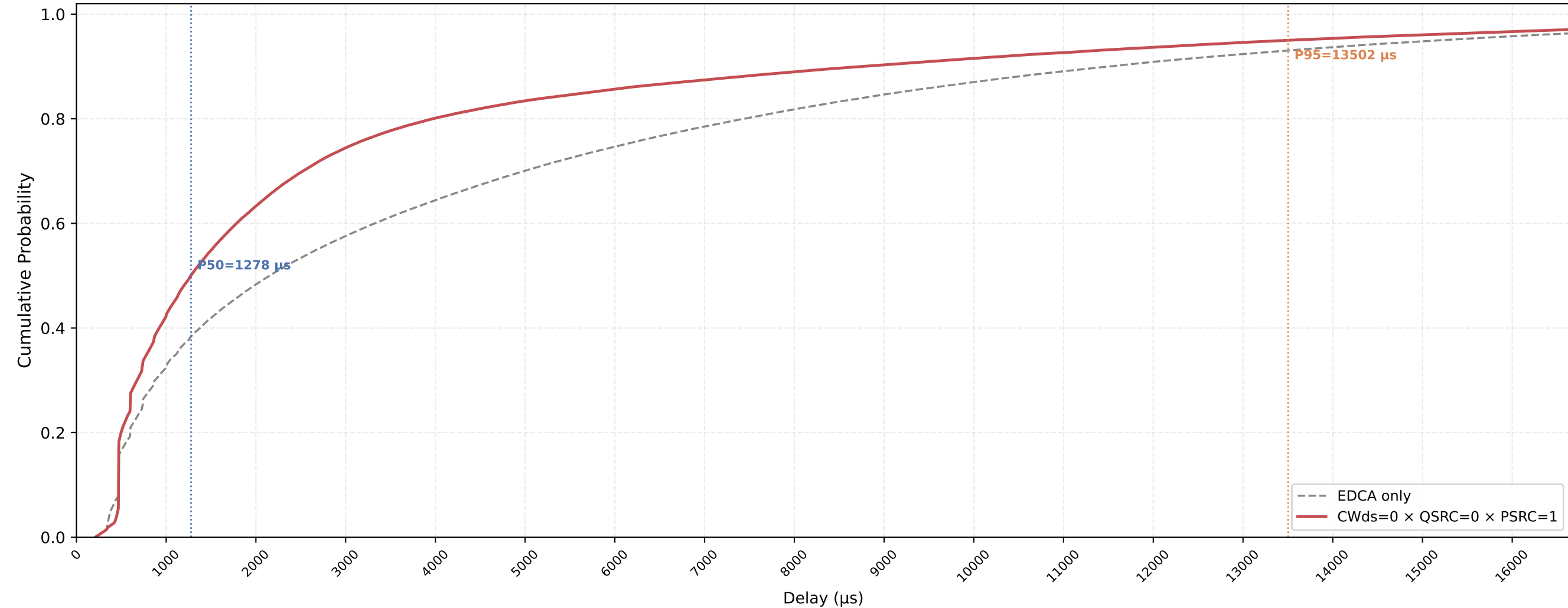
P-EDCA STA VO Delay CDF — CWds=0 × QSRC=0 × PSRC=1 nSta=30, nPedca=15, 1Mbps, avg of 10 runs
