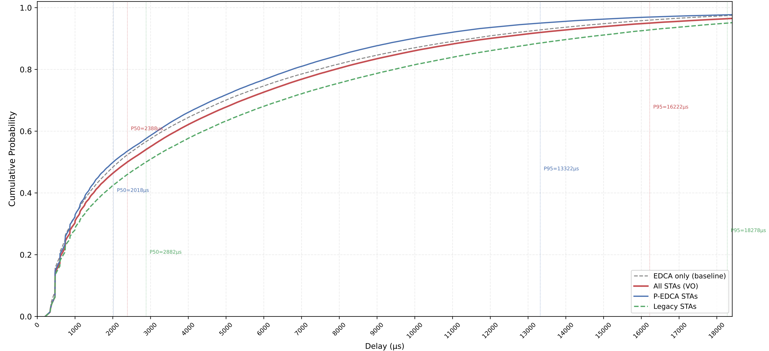
VO Delay CDF — P-EDCA / Legacy / All | CWds=0 × QSRC=3 × PSRC=3 nSta=30, nPedca=15/30, 1Mbps, avg of 10 runs
