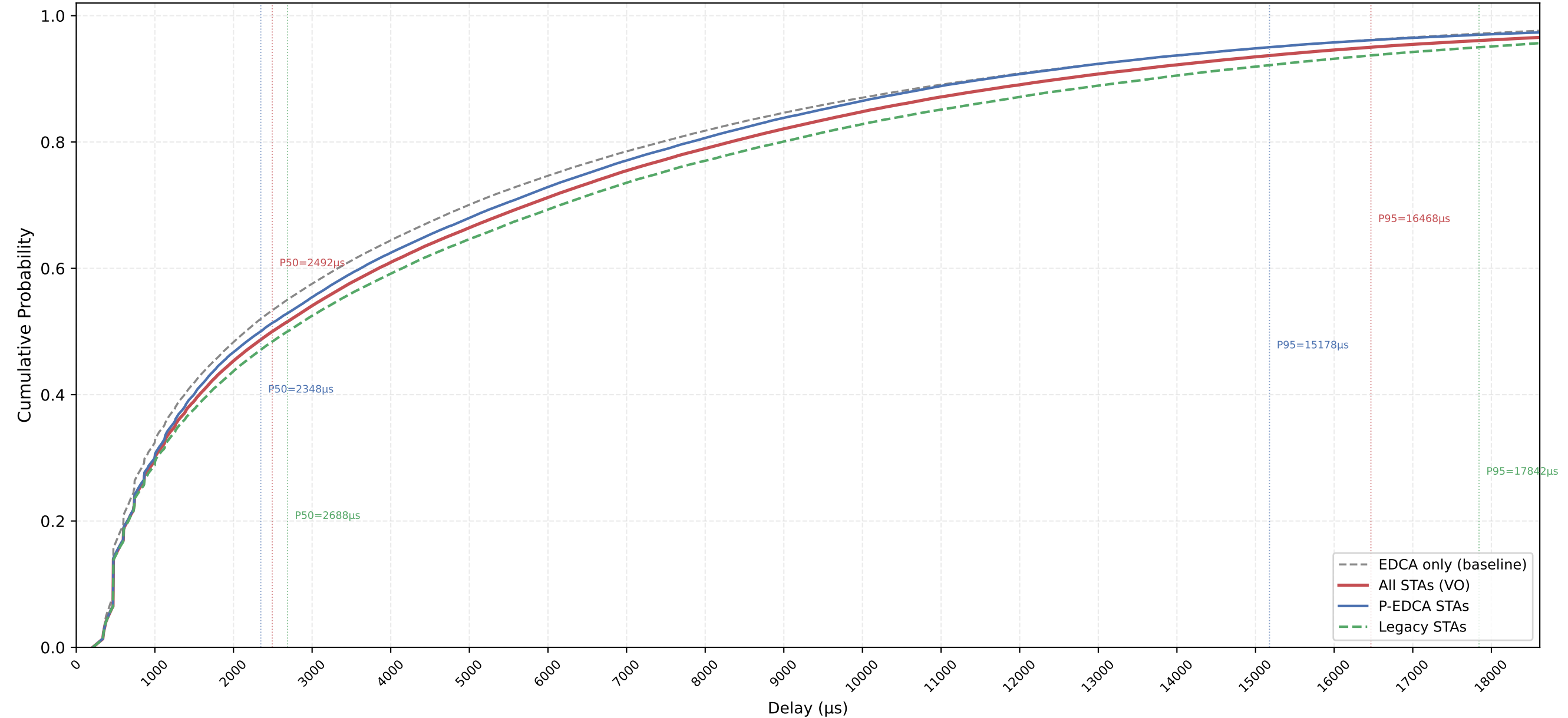
VO Delay CDF — P-EDCA / Legacy / All | CWds=0 × QSRC=4 × PSRC=3 nSta=30, nPedca=15/30, 1Mbps, avg of 10 runs
