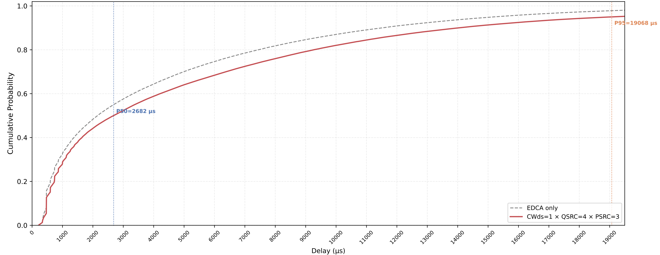
P-EDCA STA VO Delay CDF — CWds=1 × QSRC=4 × PSRC=3 nSta=30, nPedca=30, 1Mbps, avg of 10 runs
