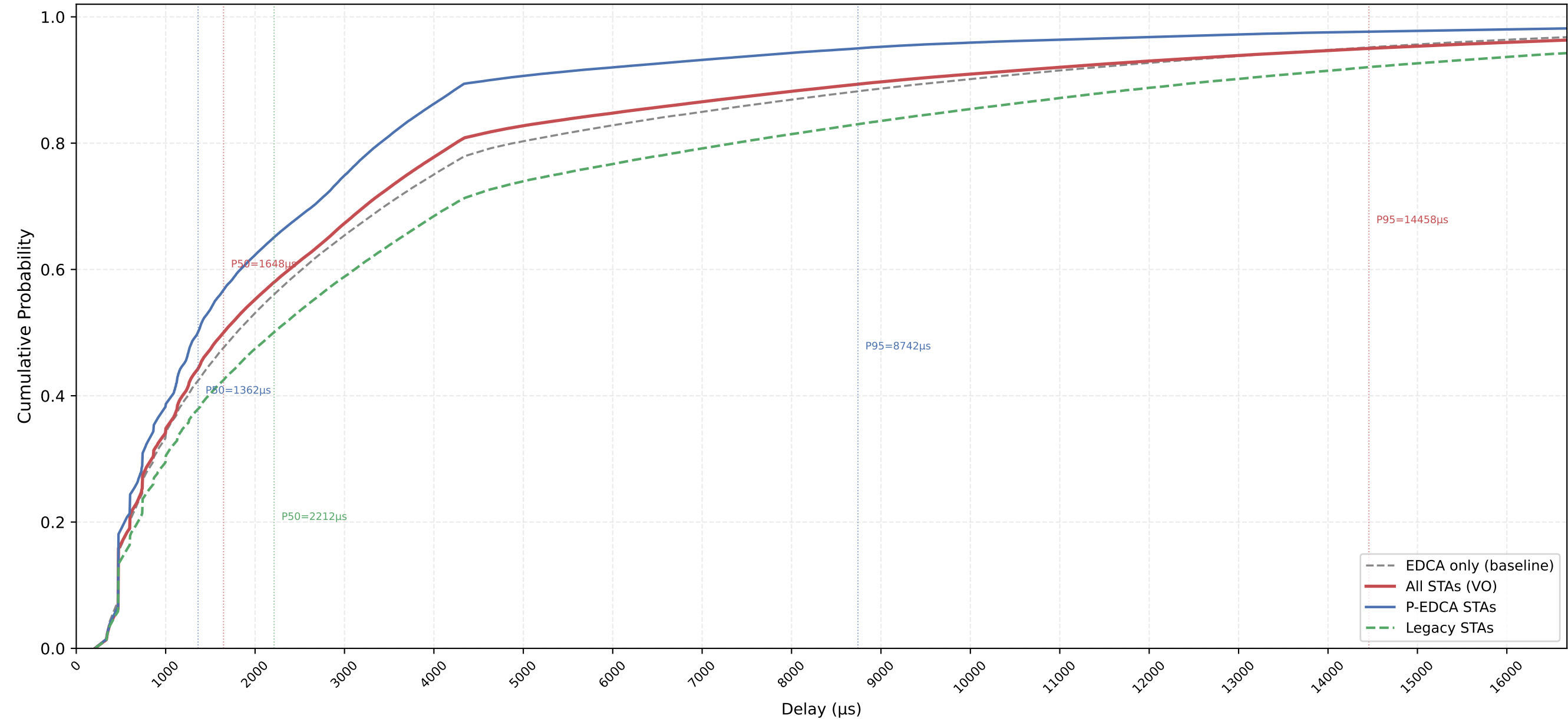
VO Delay CDF — P-EDCA / Legacy / All | CWds=0 × QSRC=2 × PSRC=2 nSta=30, nPedca=15/30, 1Mbps, avg of 10 runs
