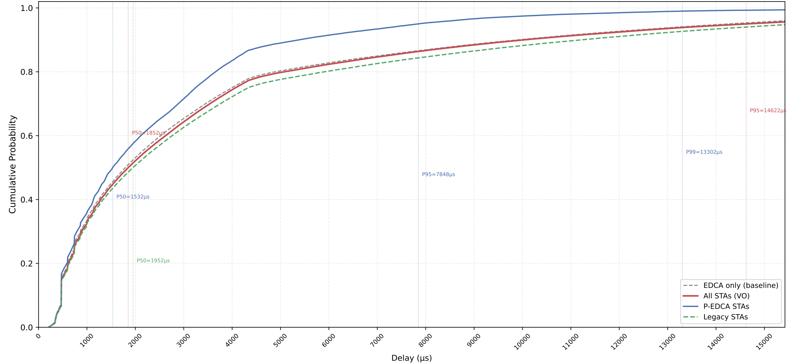
VO Delay CDF — P-EDCA / Legacy / All | CWds=0 × QSRC=3 × PSRC=3 nSta=30, nPedca=5/30, 1Mbps, avg of 10 runs
