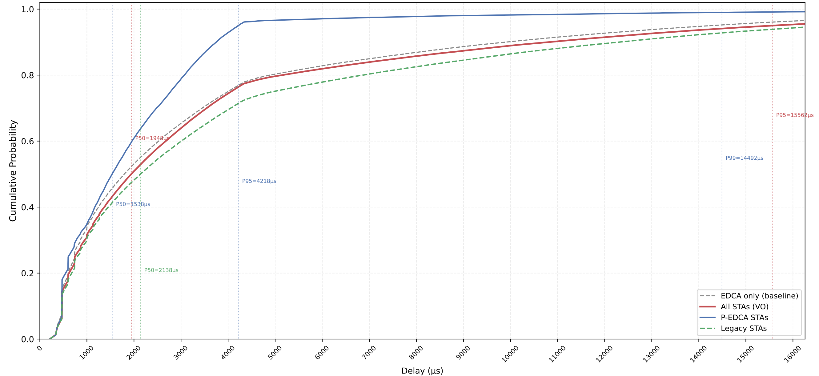
VO Delay CDF — P-EDCA / Legacy / All | CWds=1 × QSRC=1 × PSRC=2 nSta=30, nPedca=5/30, 1Mbps, avg of 10 runs
