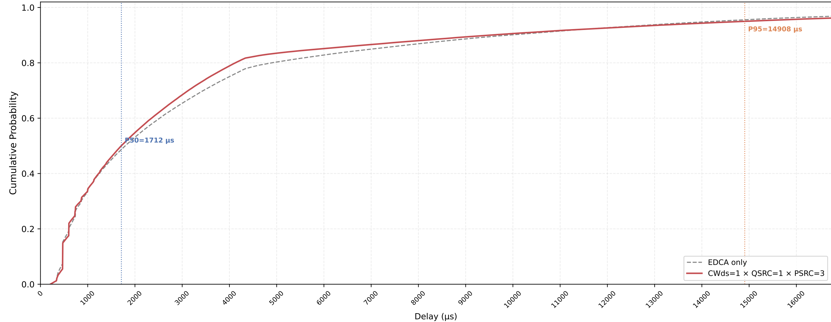
VO (all STAs) Delay CDF — CWds=1 × QSRC=1 × PSRC=3 nSta=30, nPedca=15, 1Mbps, avg of 10 runs
