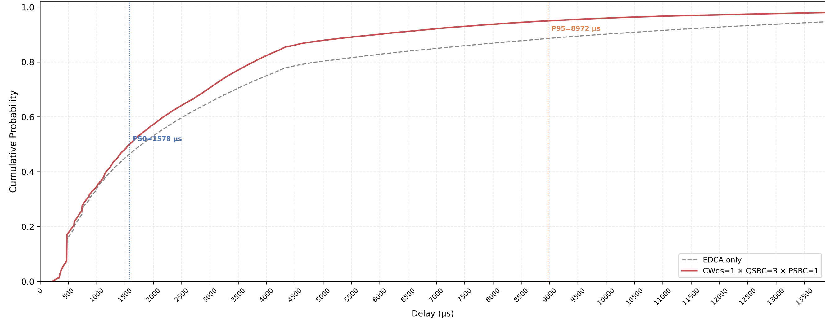
P-EDCA STA VO Delay CDF — CWds=1 × QSRC=3 × PSRC=1 nSta=30, nPedca=5, 1Mbps, avg of 10 runs
