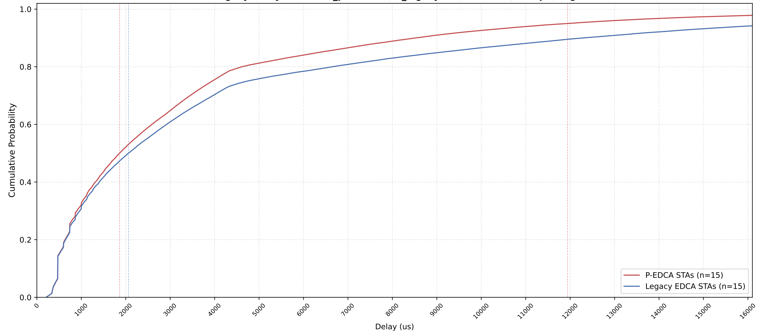
P-EDCA vs Legacy Delay CDF — n_pedca=15, n_legacy=15, nSta=30, 1Mbps, avg of 10 runs
