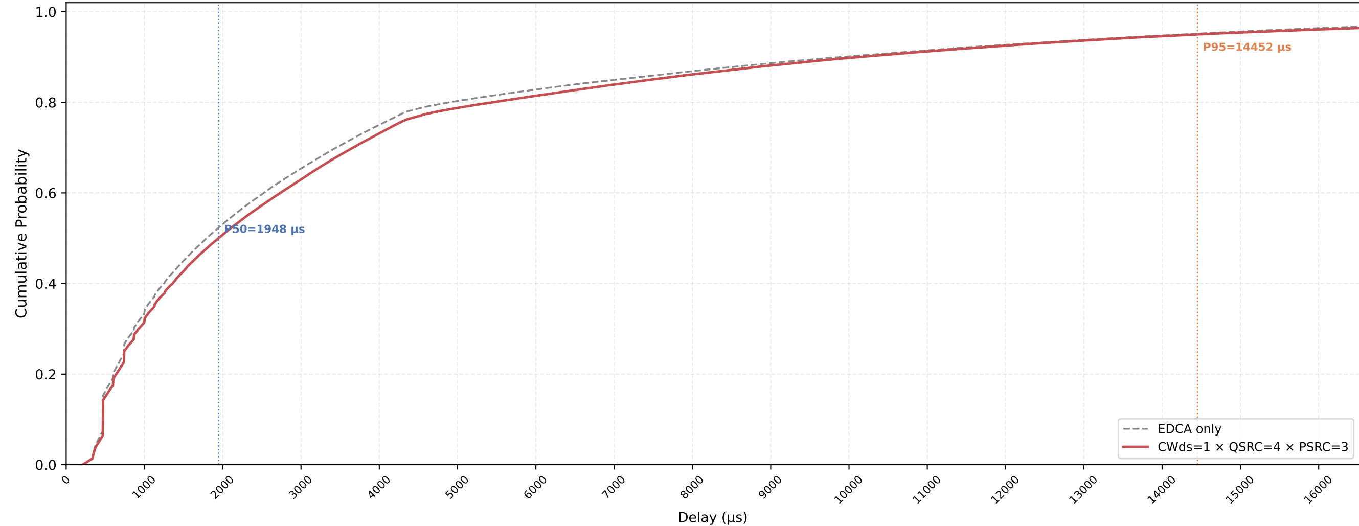
VO (all STAs) Delay CDF — CWds=1 × QSRC=4 × PSRC=3 nSta=30, nPedca=15, 1Mbps, avg of 10 runs
