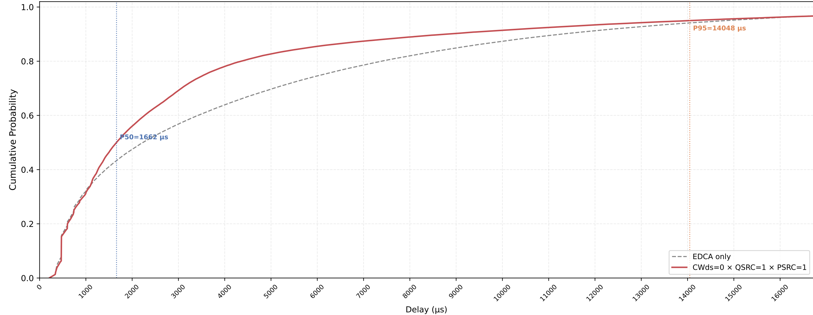
P-EDCA STA VO Delay CDF — CWds=0 × QSRC=1 × PSRC=1 nSta=30, nPedca=15, 1Mbps, avg of 10 runs
