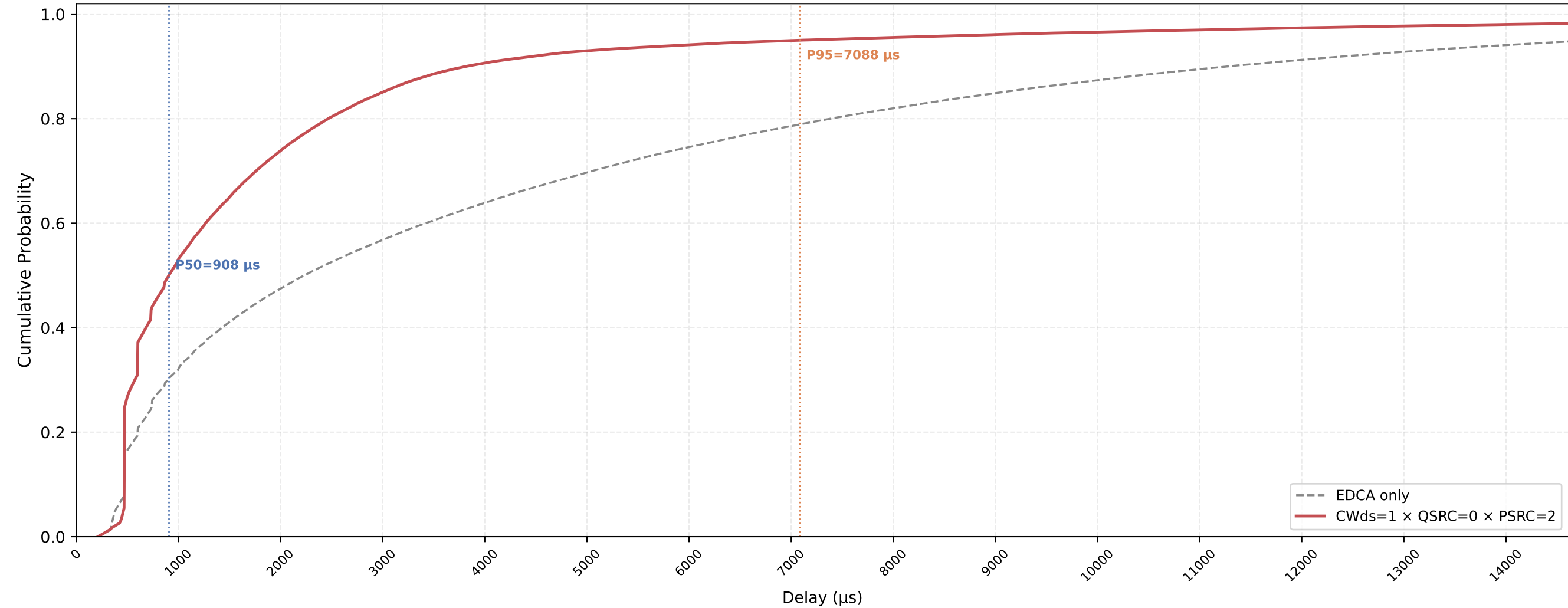
P-EDCA STA VO Delay CDF — CWds=1 × QSRC=0 × PSRC=2 nSta=30, nPedca=15, 1Mbps, avg of 10 runs
