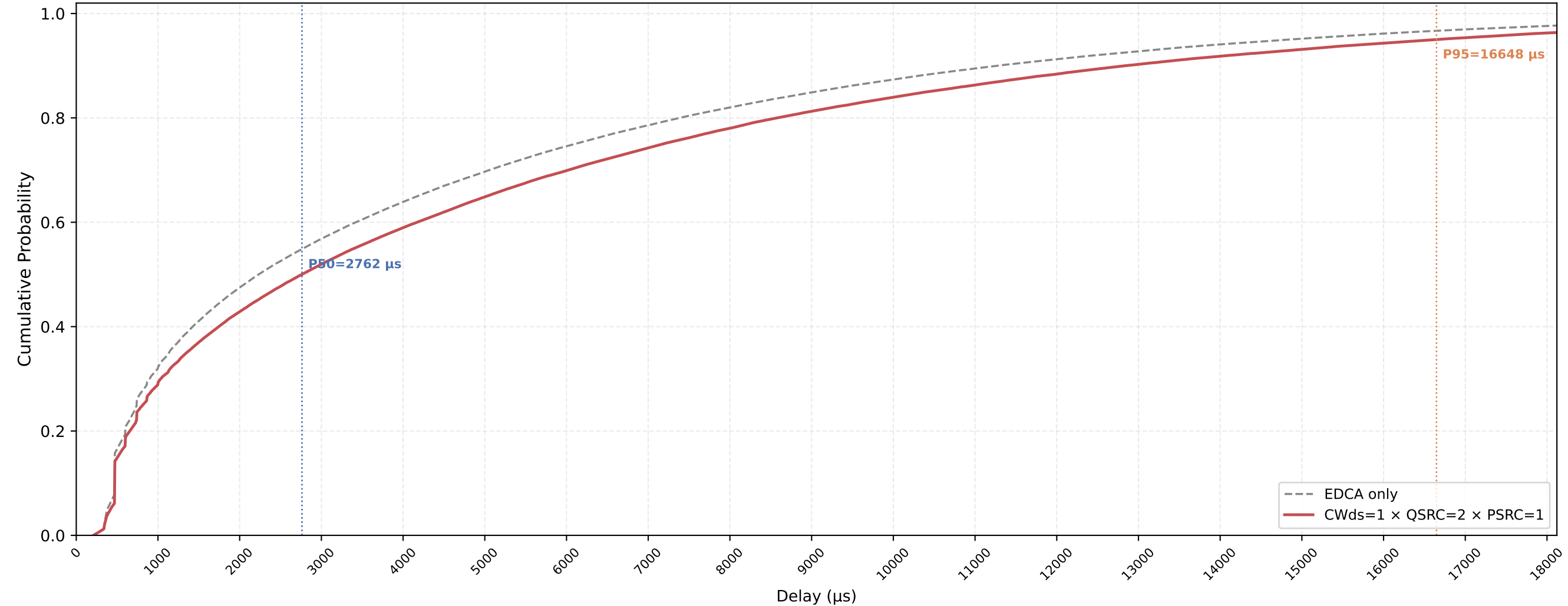
Legacy STA VO Delay CDF — CWds=1 × QSRC=2 × PSRC=1 nSta=30, nPedca=15, 1Mbps, avg of 10 runs
