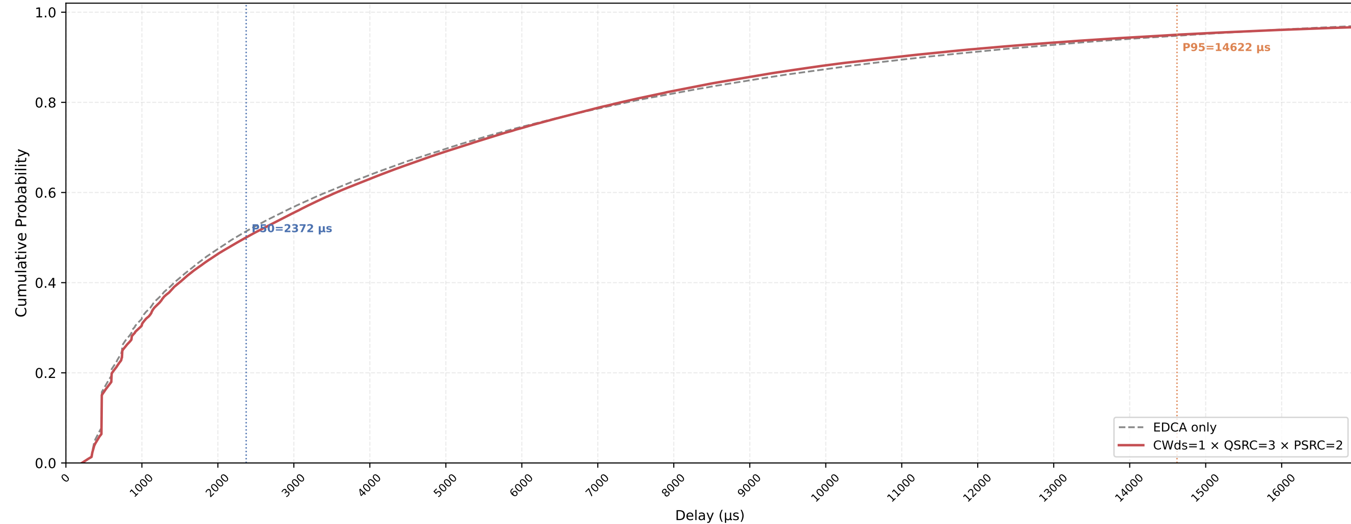
VO (all STAs) Delay CDF — CWds=1 × QSRC=3 × PSRC=2 nSta=30, nPedca=15, 1Mbps, avg of 10 runs
