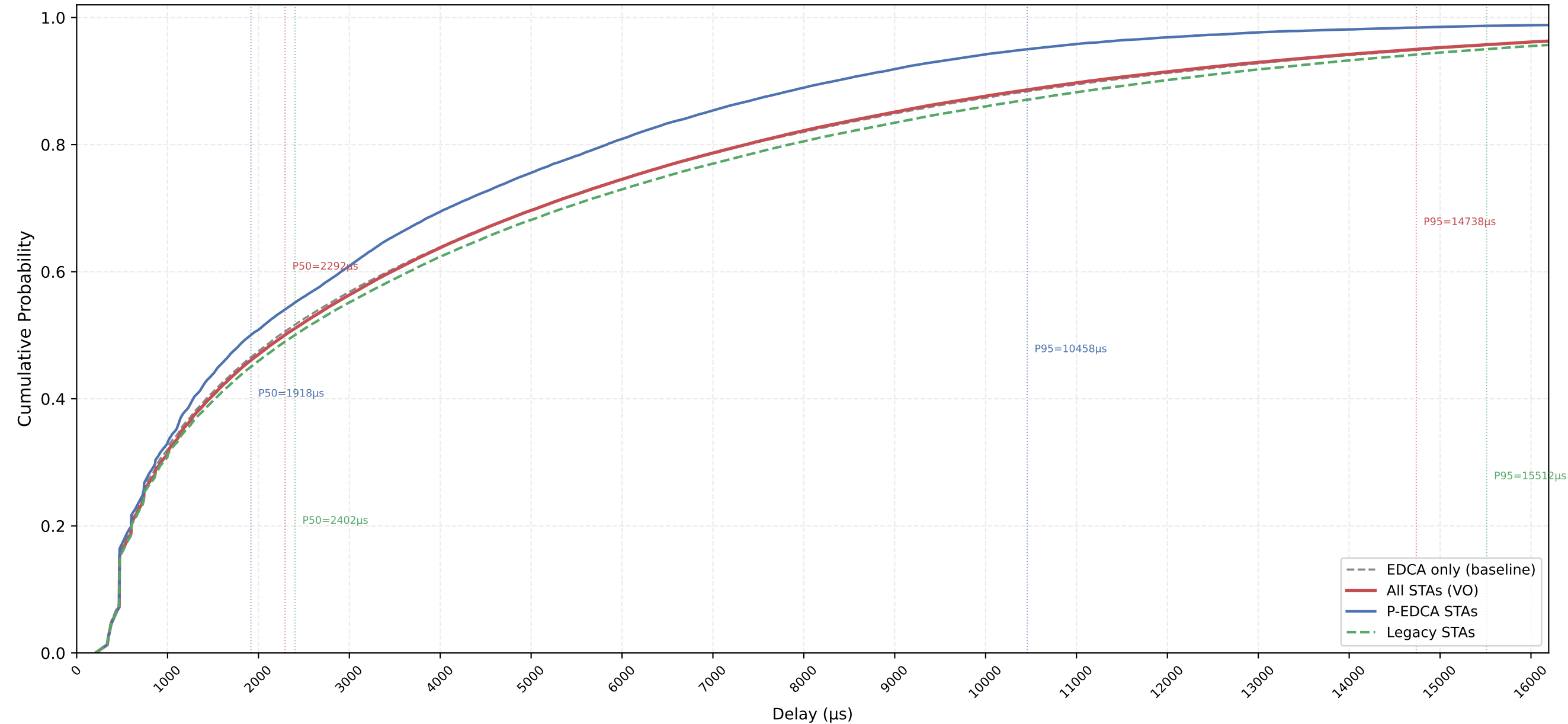
VO Delay CDF — P-EDCA / Legacy / All | CWds=1 × QSRC=3 × PSRC=3 nSta=30, nPedca=5/30, 1Mbps, avg of 10 runs
