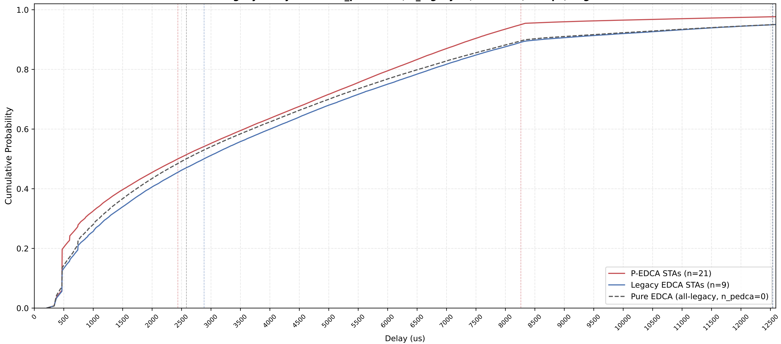
P-EDCA vs Legacy Delay CDF — n_pedca=21, n_legacy=9, nSta=30, 1Mbps, avg of 10 runs
