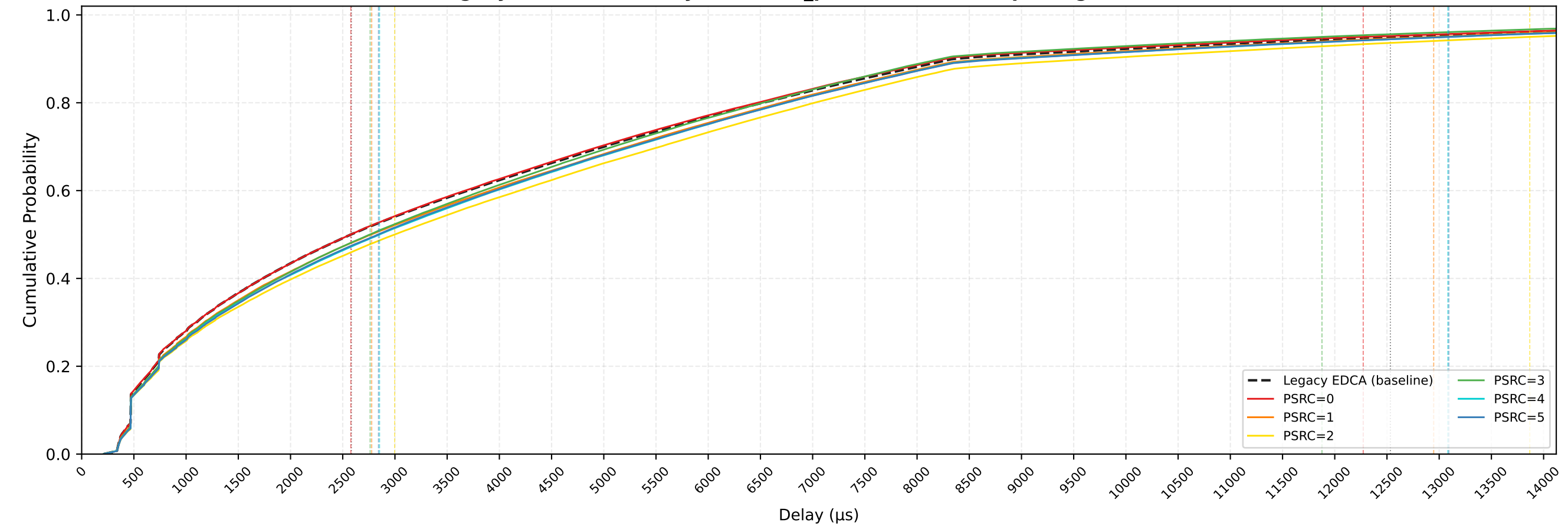
Legacy EDCA STAs Delay CDF — n_pedca=10/30, 1Mbps, avg of 10 runs
