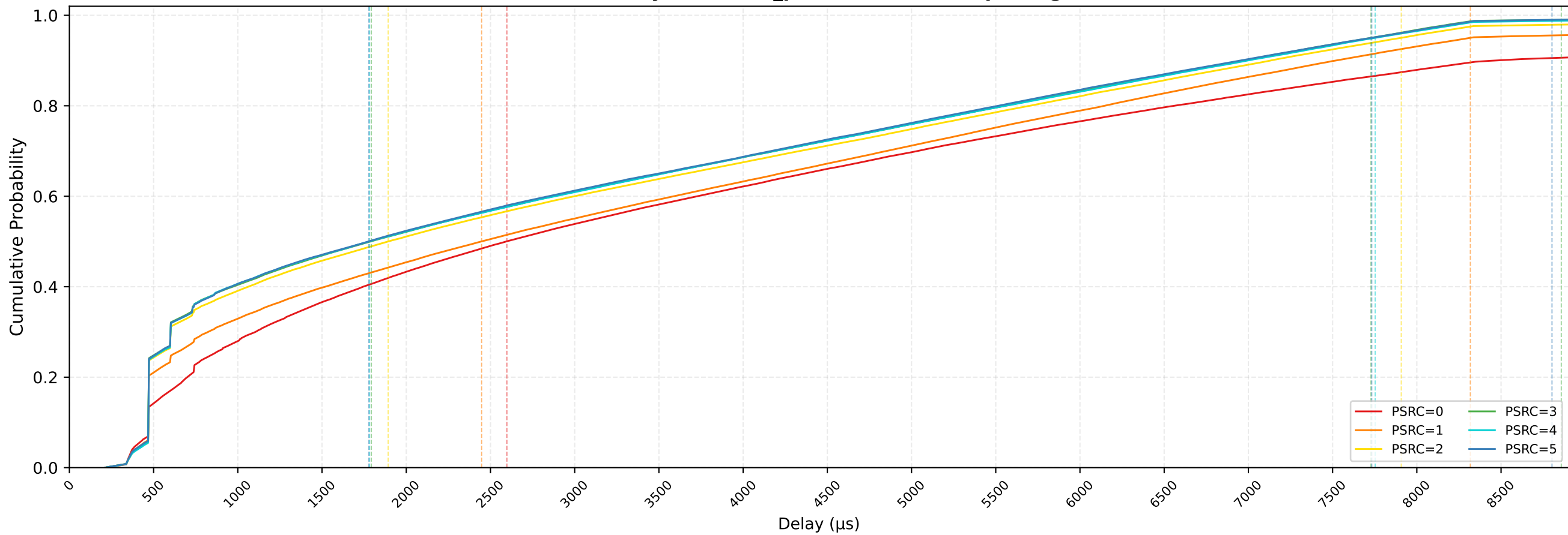
P-EDCA STAs Delay CDF — n_pedca=15/30, 1Mbps, avg of 10 runs
