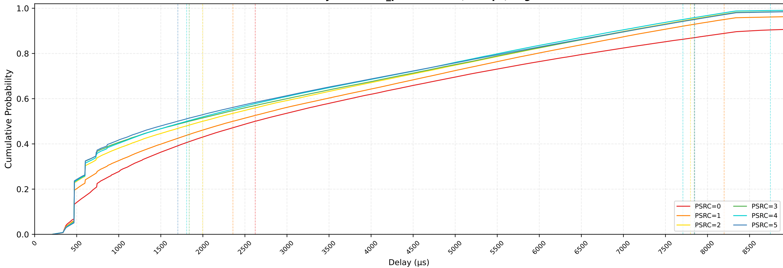
P-EDCA STAs Delay CDF — n_pedca=20/30, 1Mbps, avg of 10 runs
