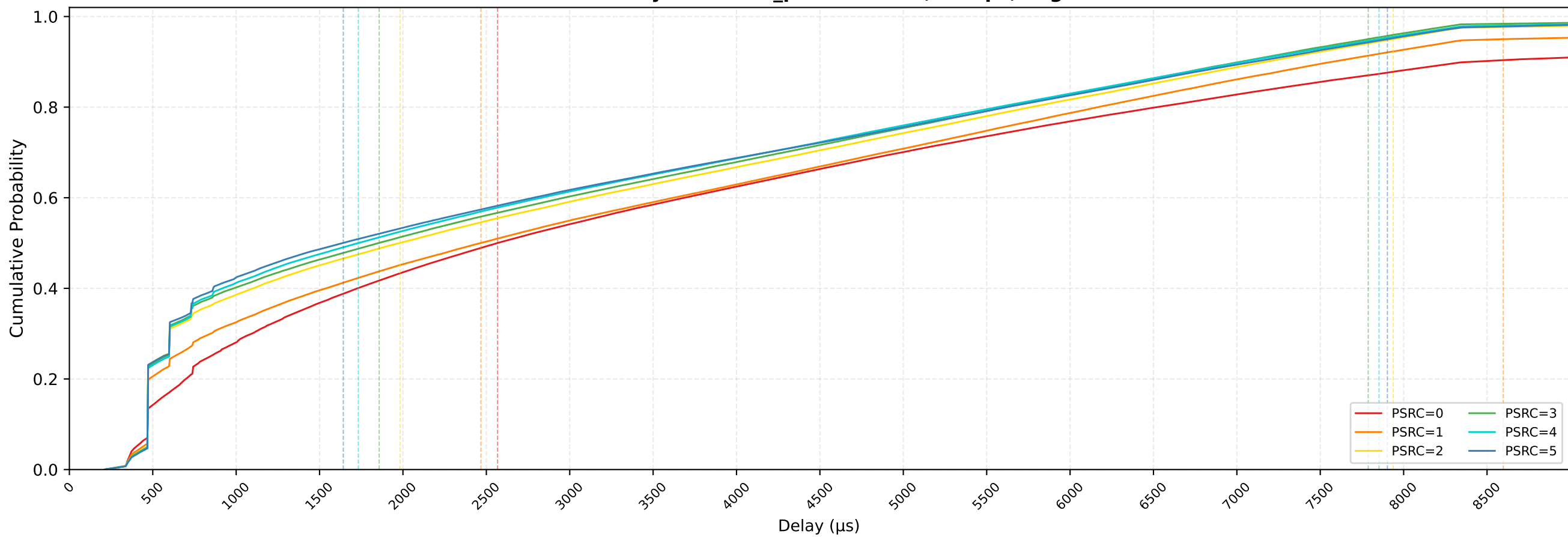
P-EDCA STAs Delay CDF — n_pedca=25/30, 1Mbps, avg of 10 runs
