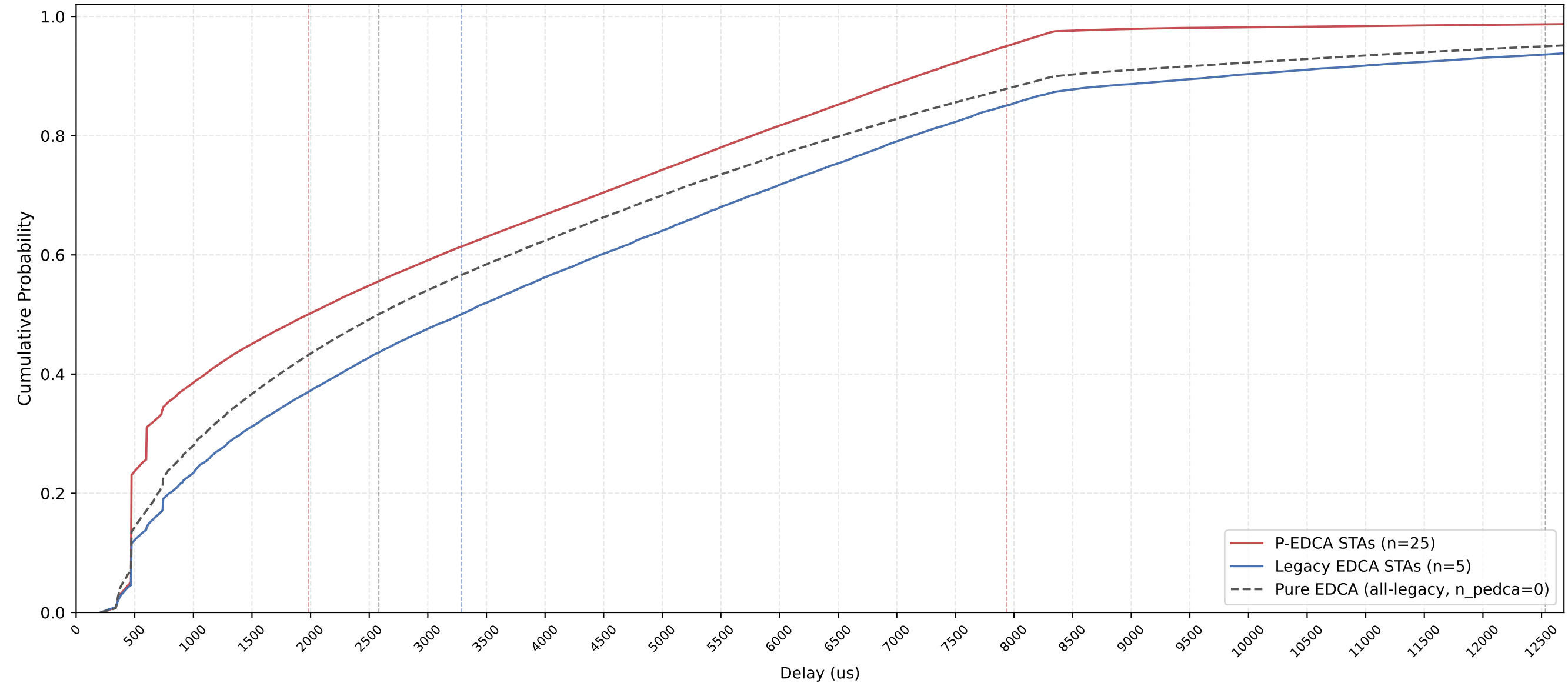
P-EDCA vs Legacy Delay CDF — n_pedca=25, n_legacy=5, nSta=30, 1Mbps, avg of 10 runs
