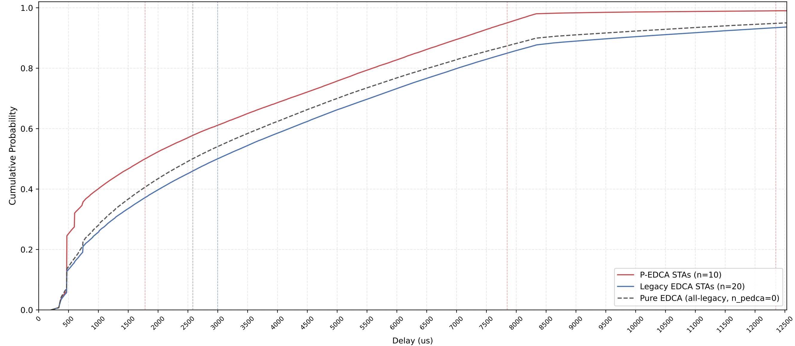
P-EDCA vs Legacy Delay CDF — n_pedca=10, n_legacy=20, nSta=30, 1Mbps, avg of 10 runs
