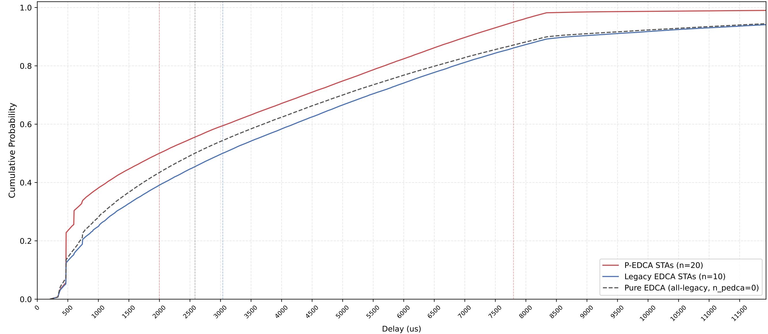
P-EDCA vs Legacy Delay CDF — n_pedca=20, n_legacy=10, nSta=30, 1Mbps, avg of 10 runs
