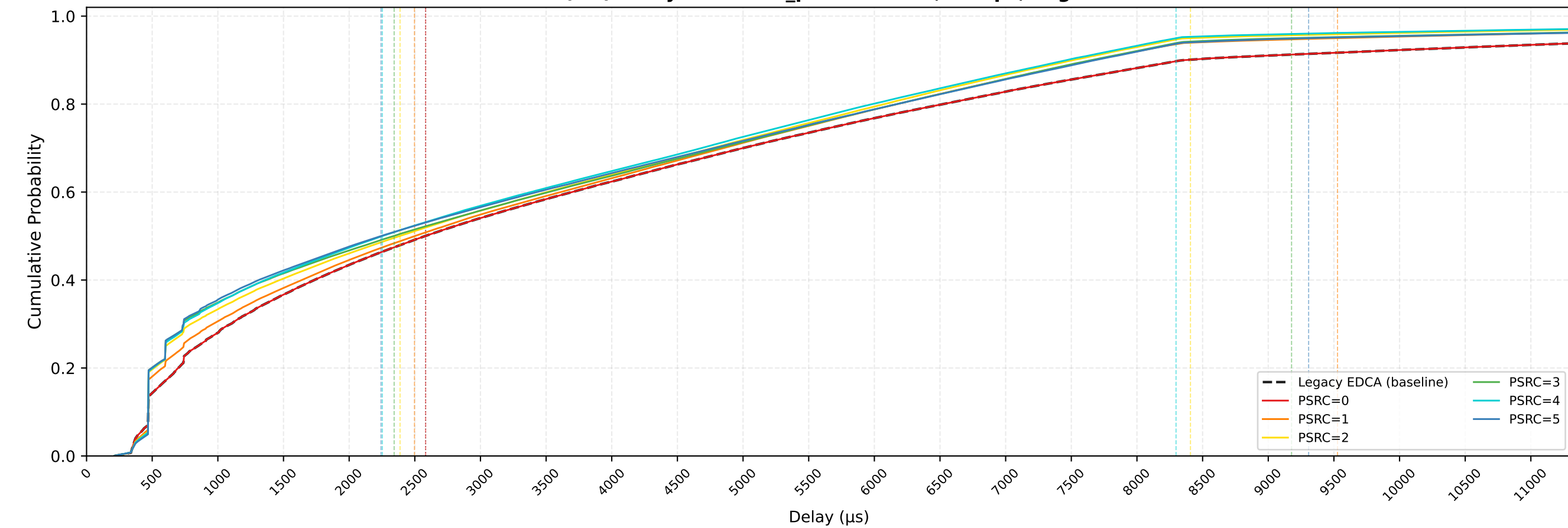
All STAs (VO) Delay CDF — n_pedca=20/30, 1Mbps, avg of 10 runs
