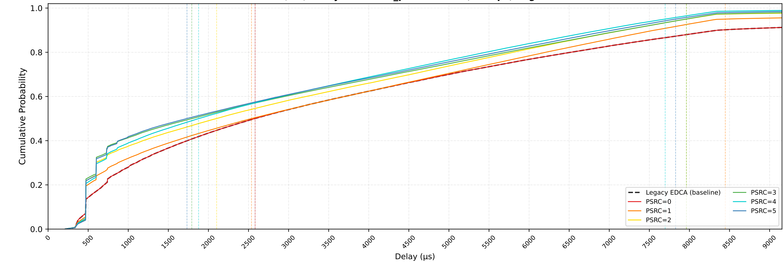
All STAs (VO) Delay CDF — n_pedca=30/30, 1Mbps, avg of 10 runs
