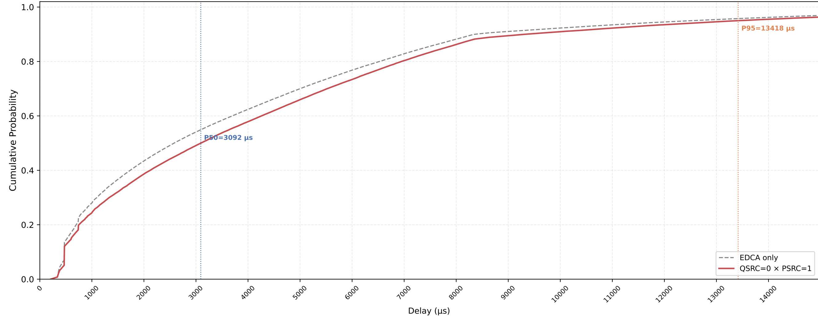
Legacy STA VO Delay CDF — QSRC=0 × PSRC=1 nSta=30, nPedca=15, 1Mbps, avg of 10 runs
