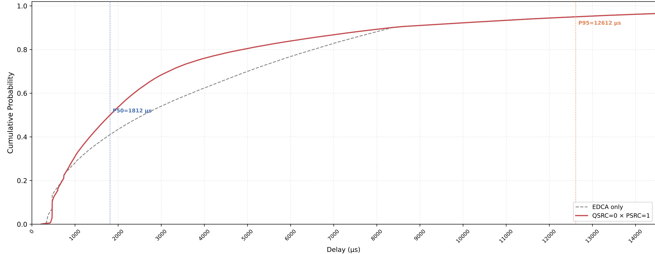
P-EDCA STA VO Delay CDF — QSRC=0 × PSRC=1 nSta=30, nPedca=30, 1Mbps, avg of 10 runs
