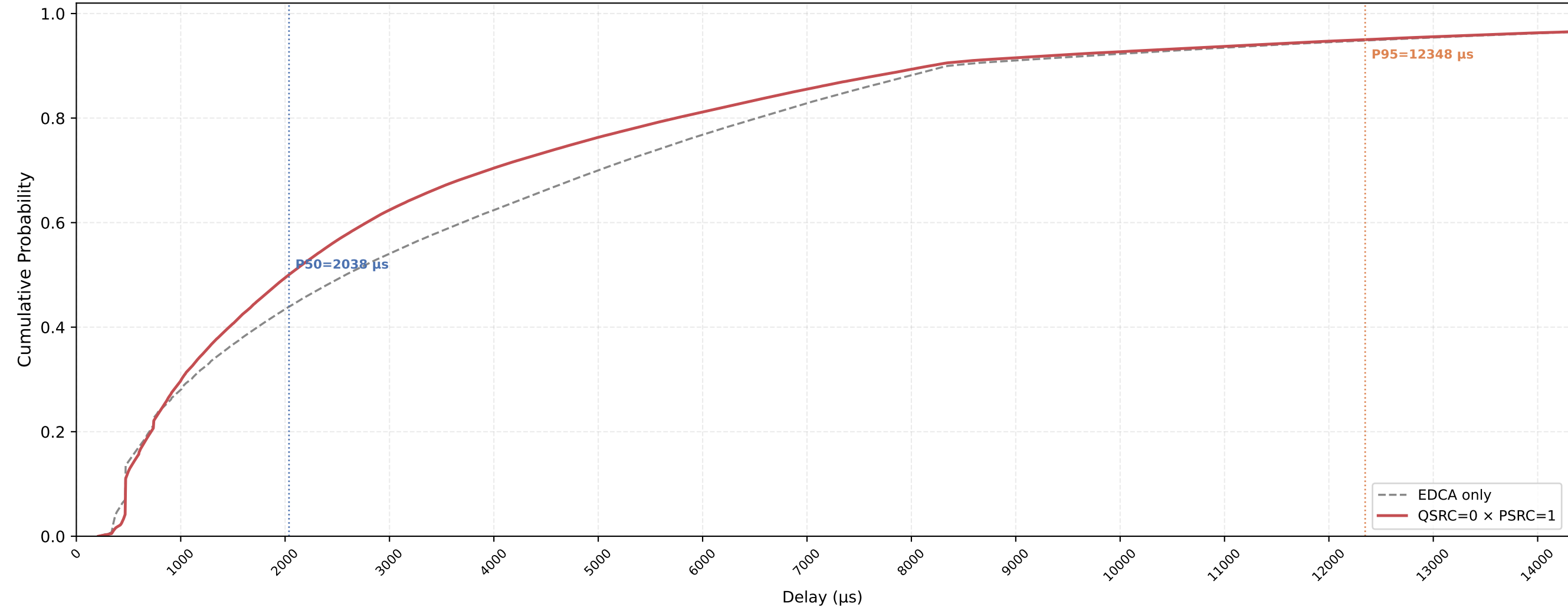
VO (all STAs) Delay CDF — QSRC=0 × PSRC=1 nSta=30, nPedca=15, 1Mbps, avg of 10 runs
