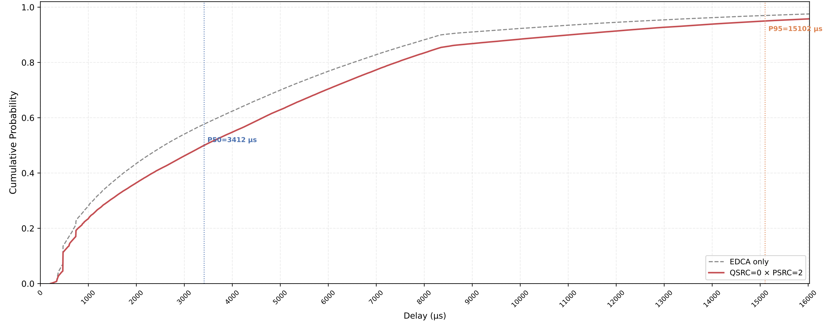
Legacy STA VO Delay CDF — QSRC=0 × PSRC=2 nSta=30, nPedca=15, 1Mbps, avg of 10 runs
