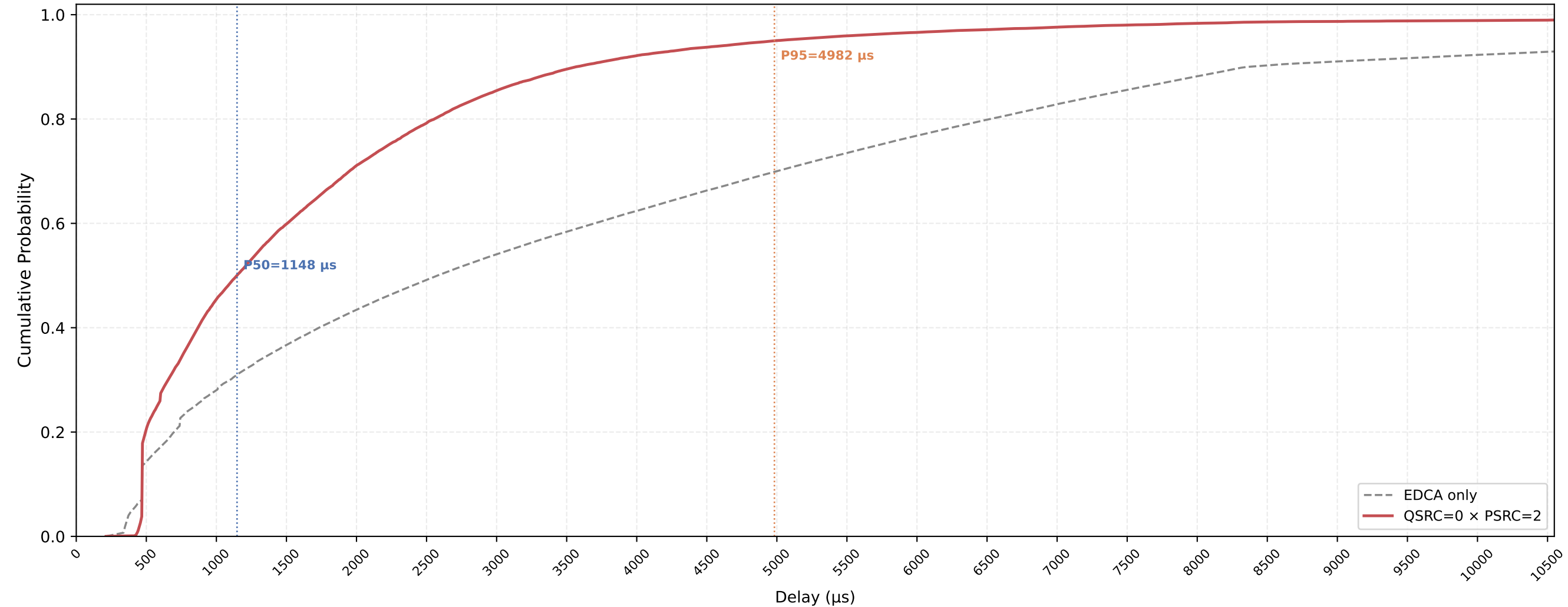
P-EDCA STA VO Delay CDF — QSRC=0 × PSRC=2 nSta=30, nPedca=5, 1Mbps, avg of 10 runs
