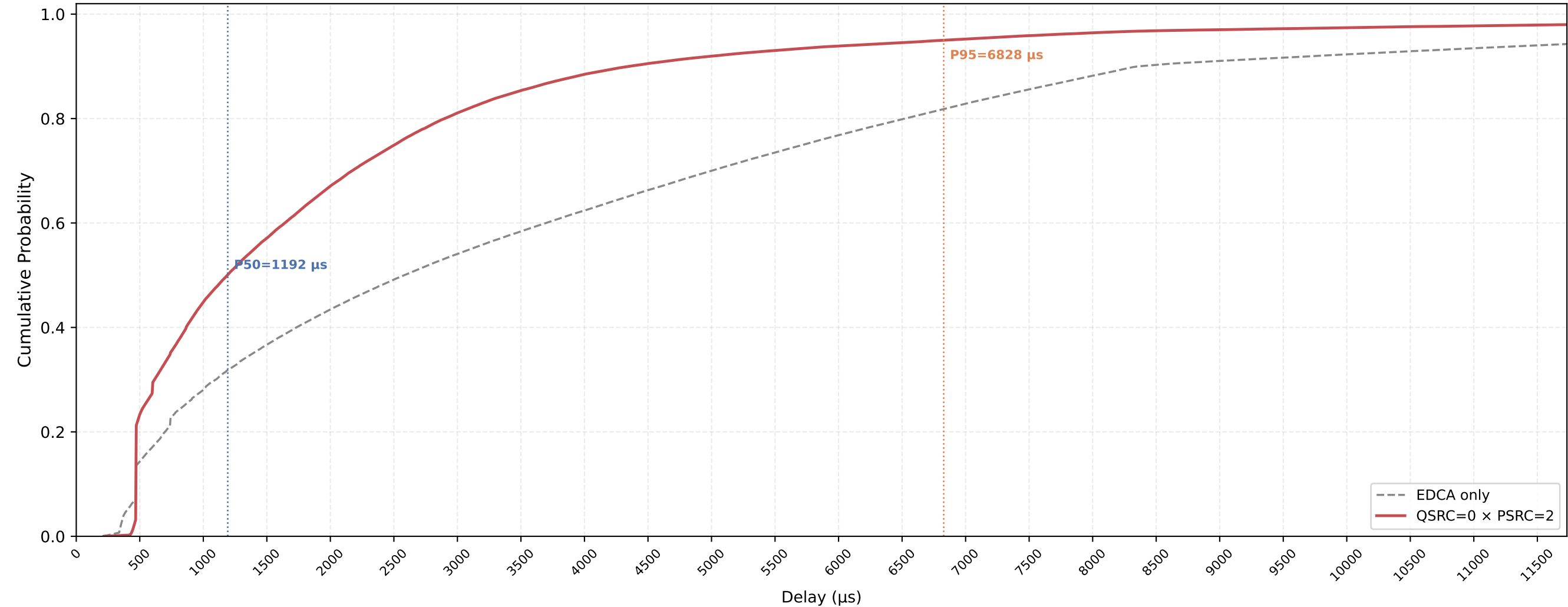
P-EDCA STA VO Delay CDF — QSRC=0 × PSRC=2 nSta=30, nPedca=15, 1Mbps, avg of 10 runs
