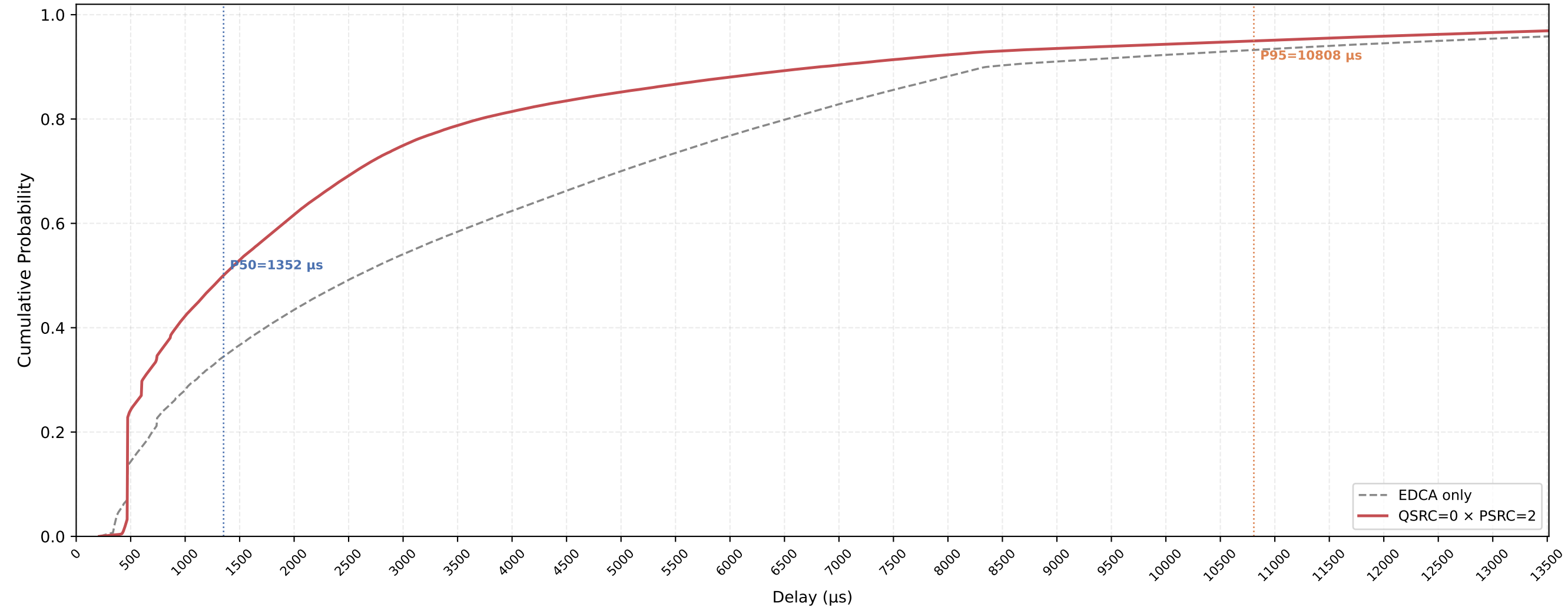
P-EDCA STA VO Delay CDF — QSRC=0 × PSRC=2 nSta=30, nPedca=30, 1Mbps, avg of 10 runs
