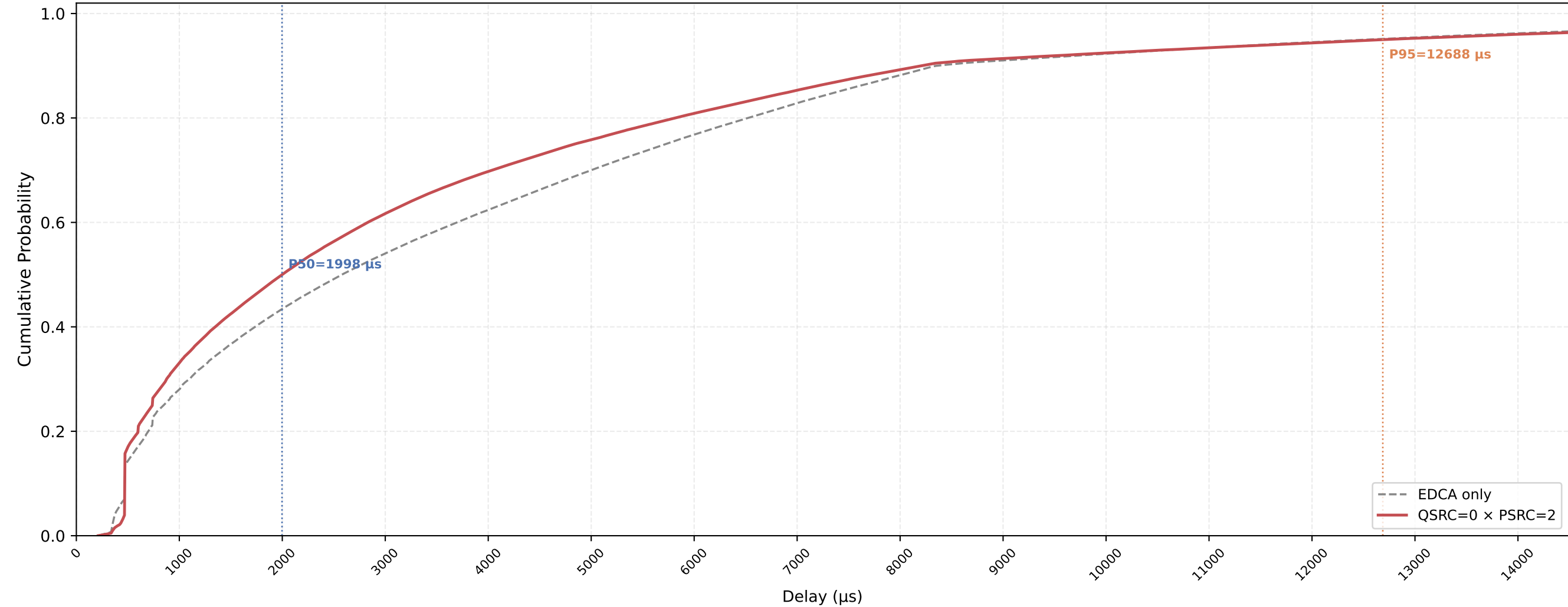
VO (all STAs) Delay CDF — QSRC=0 × PSRC=2 nSta=30, nPedca=15, 1Mbps, avg of 10 runs
