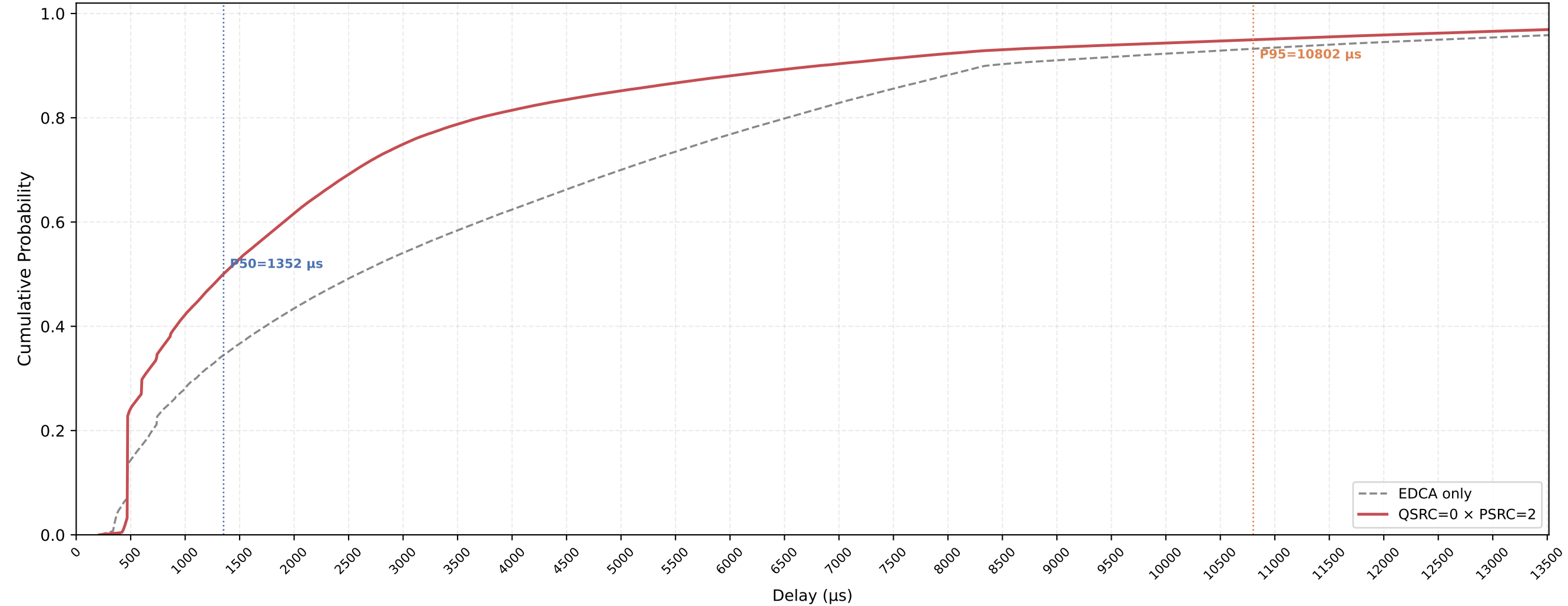
VO (all STAs) Delay CDF — QSRC=0 × PSRC=2 nSta=30, nPedca=30, 1Mbps, avg of 10 runs
