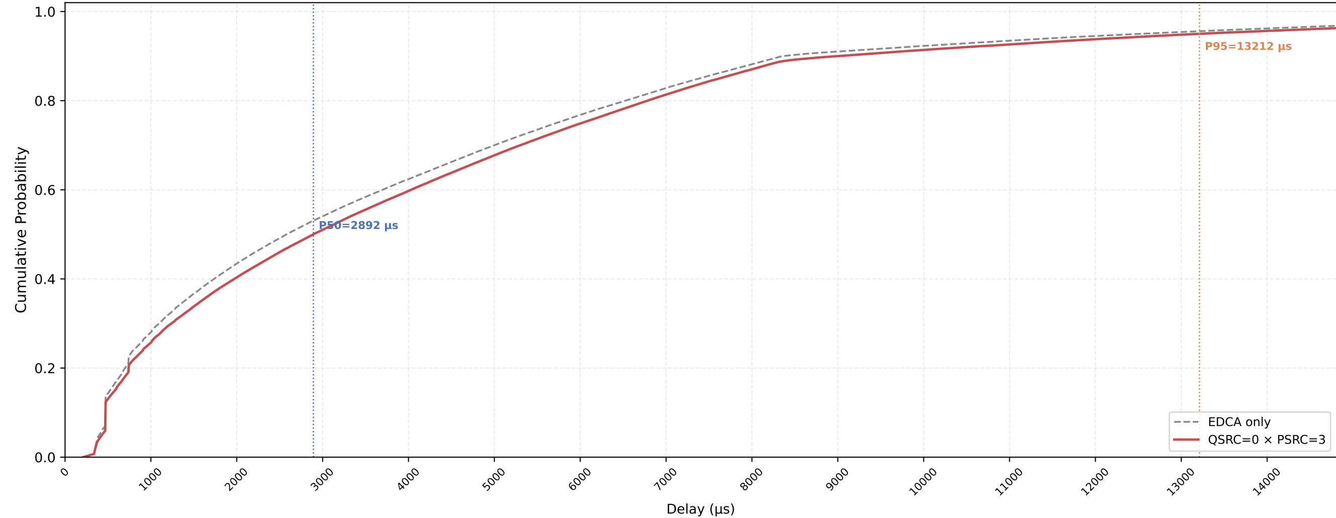
Legacy STA VO Delay CDF — QSRC=0 × PSRC=3 nSta=30, nPedca=5, 1Mbps, avg of 10 runs
