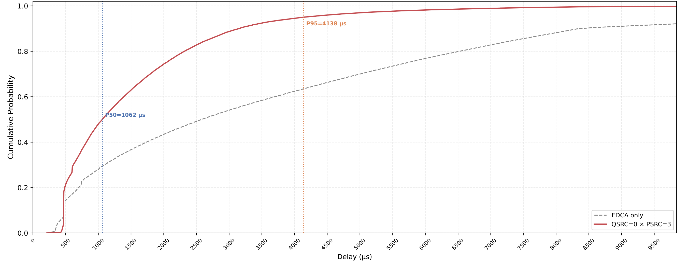
P-EDCA STA VO Delay CDF — QSRC=0 × PSRC=3 nSta=30, nPedca=5, 1Mbps, avg of 10 runs
