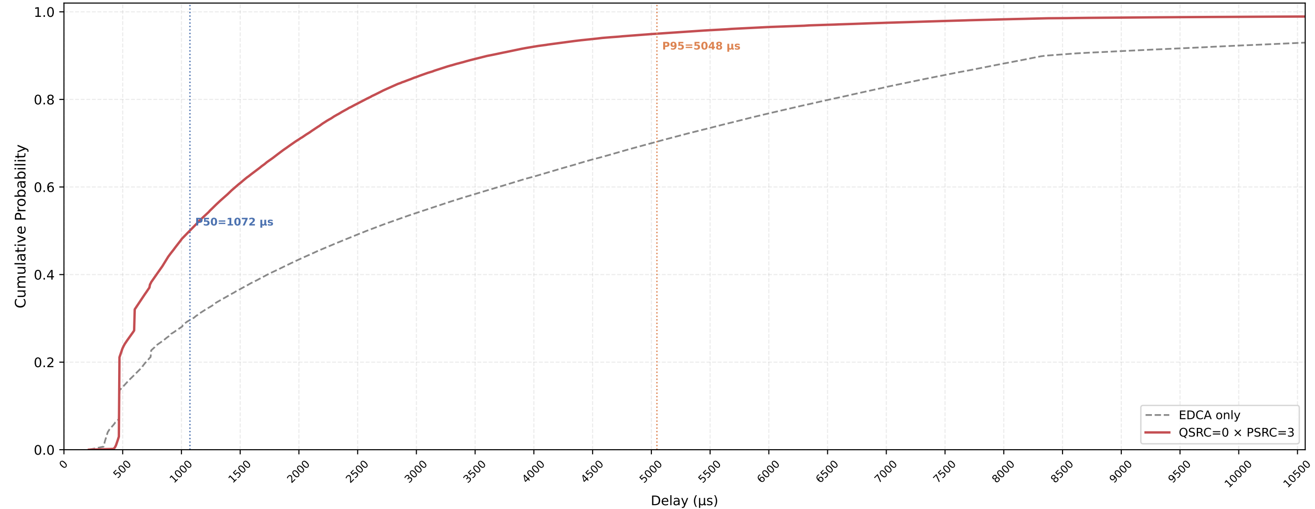
P-EDCA STA VO Delay CDF — QSRC=0 × PSRC=3 nSta=30, nPedca=15, 1Mbps, avg of 10 runs
