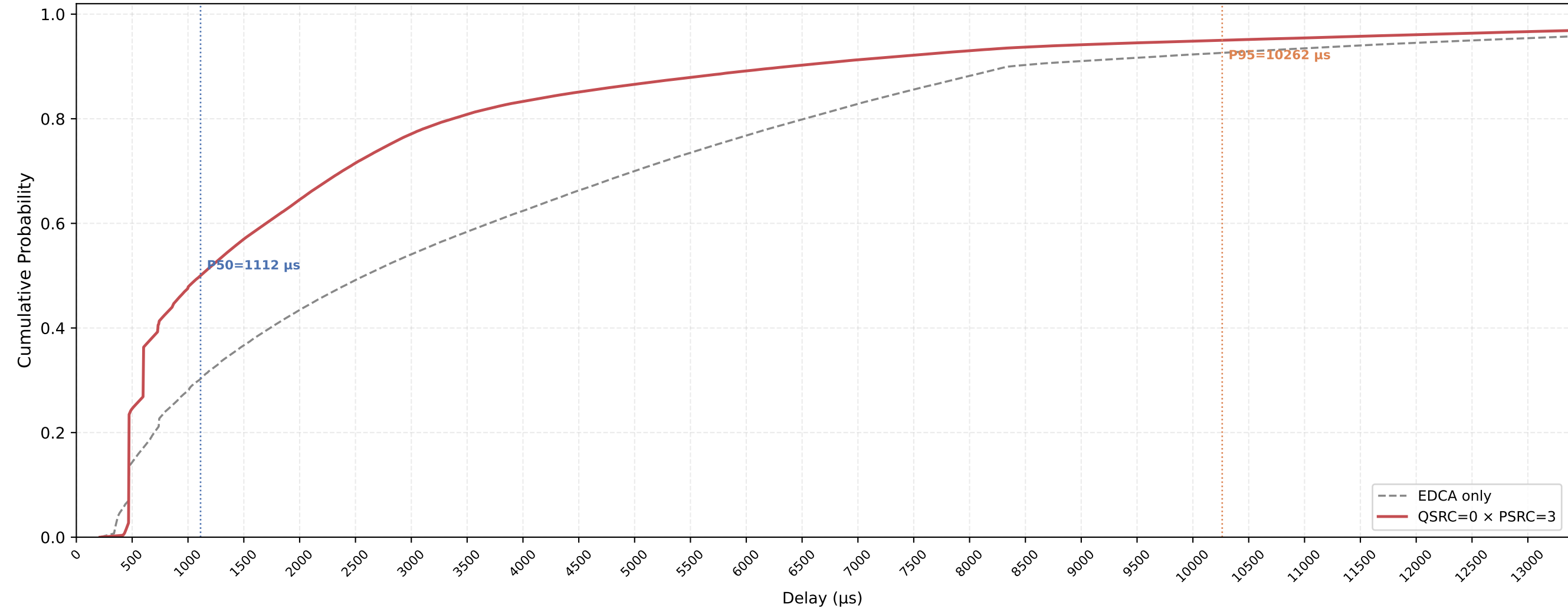
P-EDCA STA VO Delay CDF — QSRC=0 × PSRC=3 nSta=30, nPedca=30, 1Mbps, avg of 10 runs
