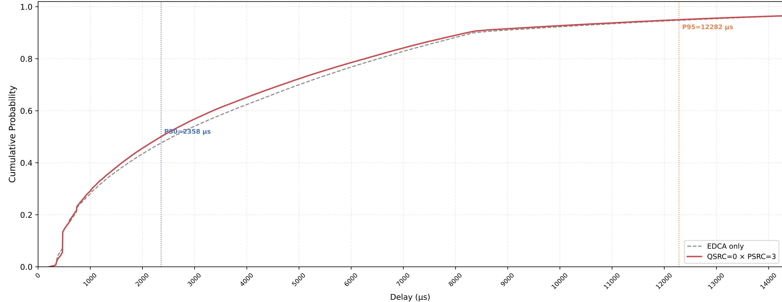
VO (all STAs) Delay CDF — QSRC=0 × PSRC=3 nSta=30, nPedca=5, 1Mbps, avg of 10 runs
