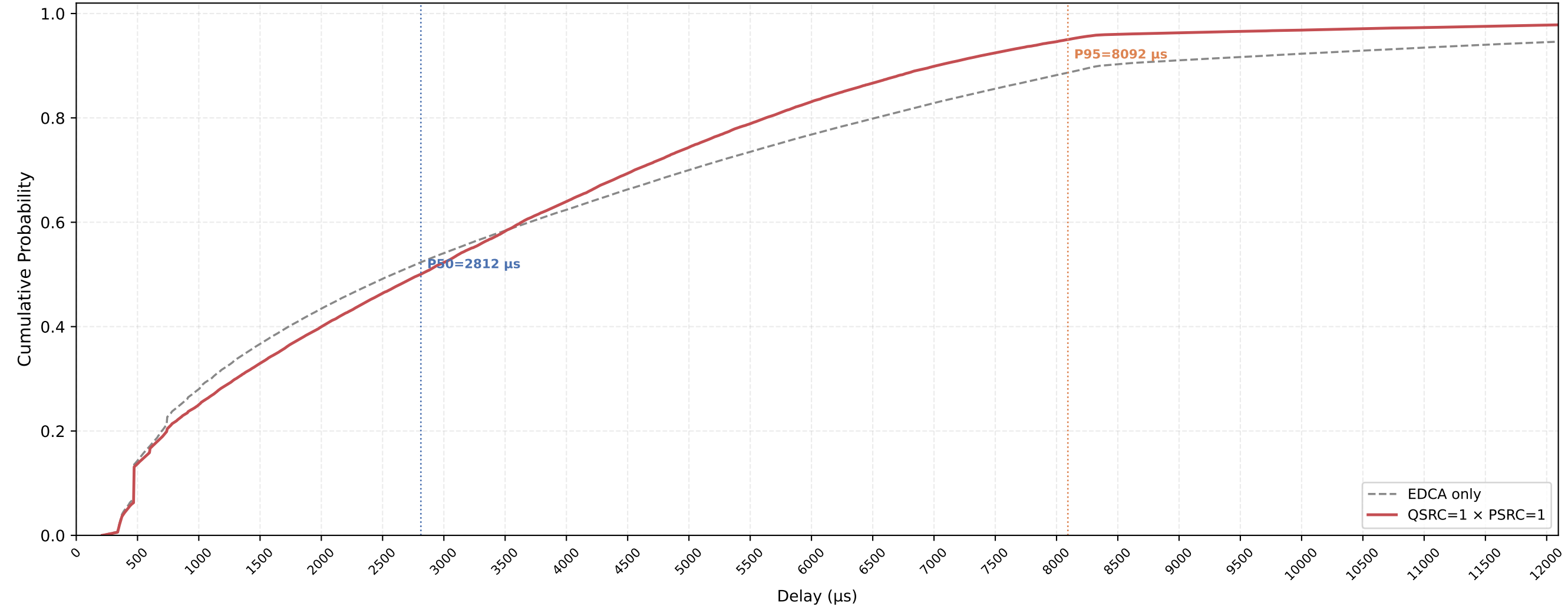
P-EDCA STA VO Delay CDF — QSRC=1 × PSRC=1 nSta=30, nPedca=5, 1Mbps, avg of 10 runs
