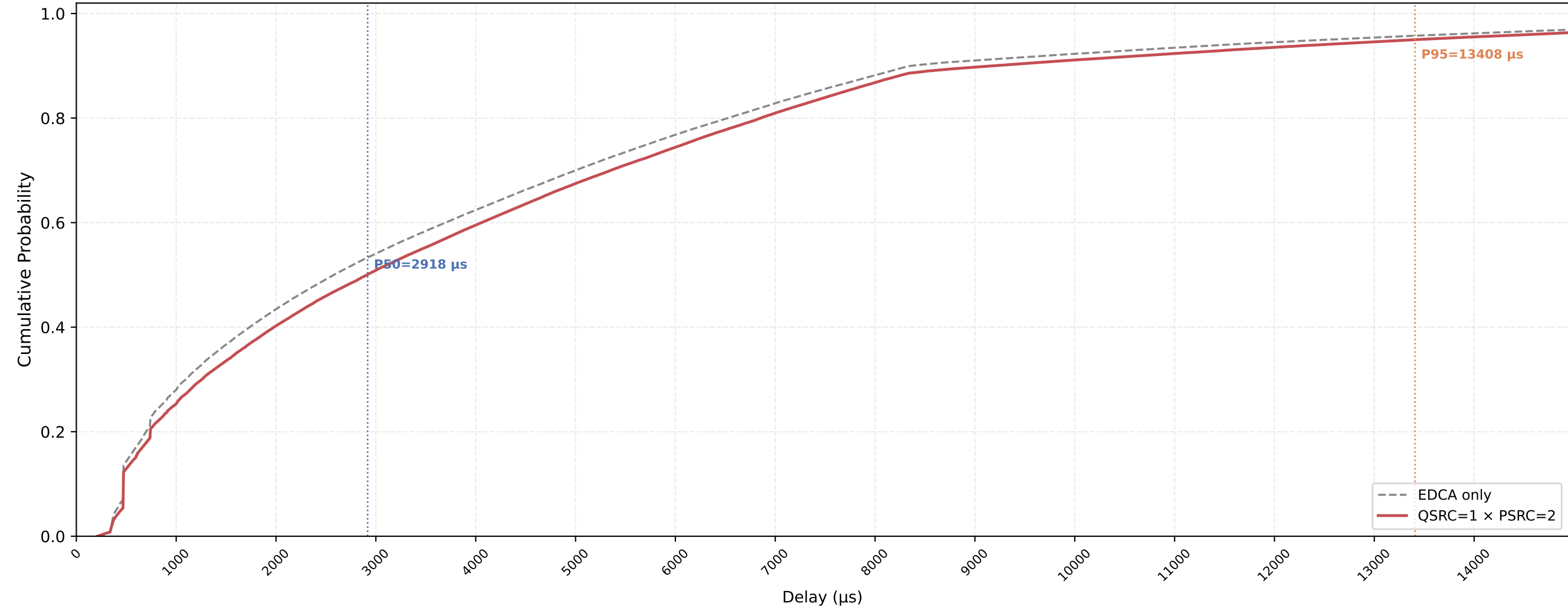
Legacy STA VO Delay CDF — QSRC=1 × PSRC=2 nSta=30, nPedca=15, 1Mbps, avg of 10 runs
