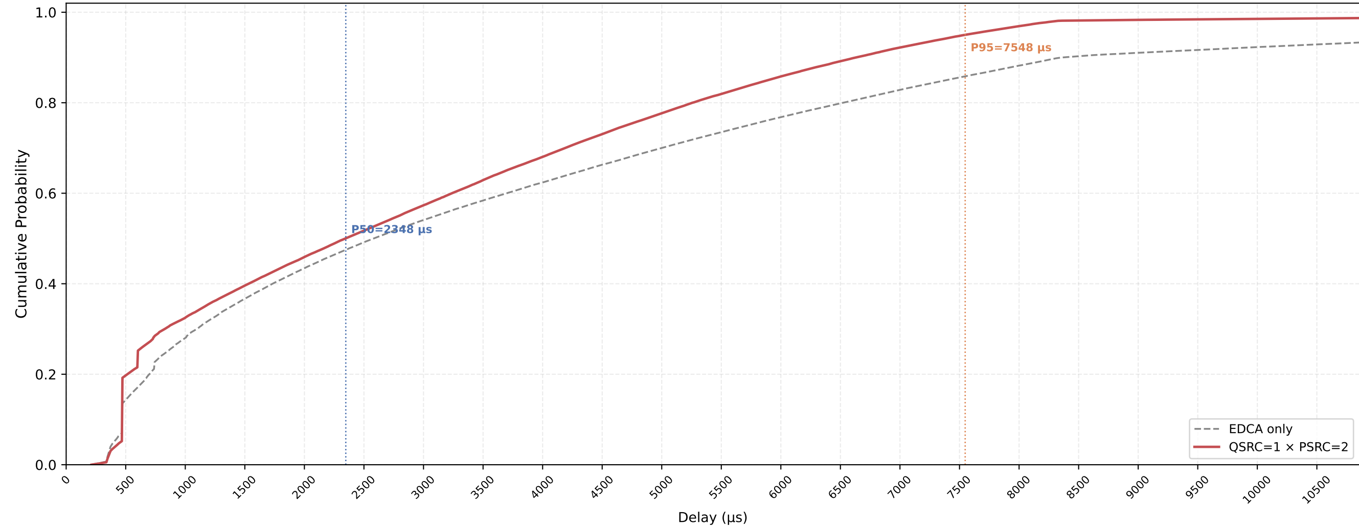
P-EDCA STA VO Delay CDF — QSRC=1 × PSRC=2 nSta=30, nPedca=15, 1Mbps, avg of 10 runs
